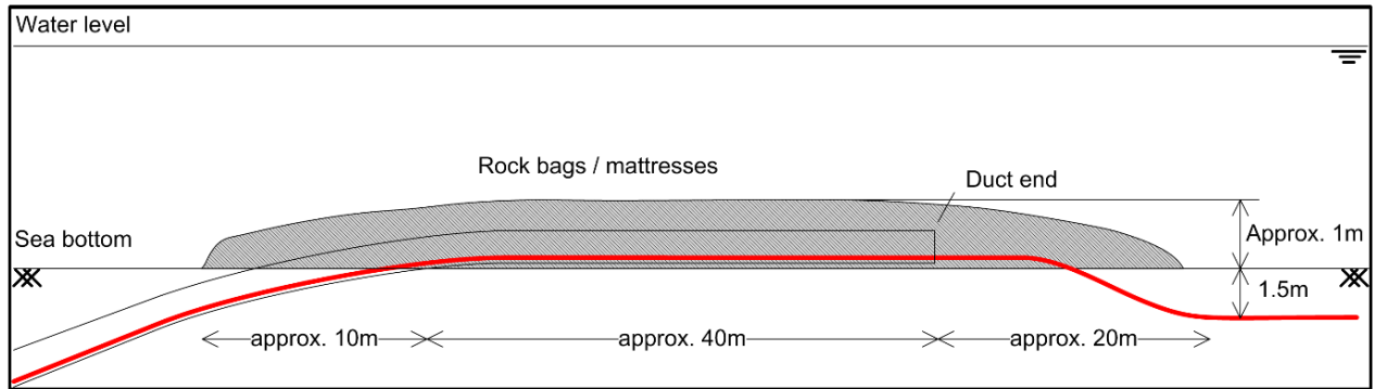
Figure 19 Indicative duct and cable protection
