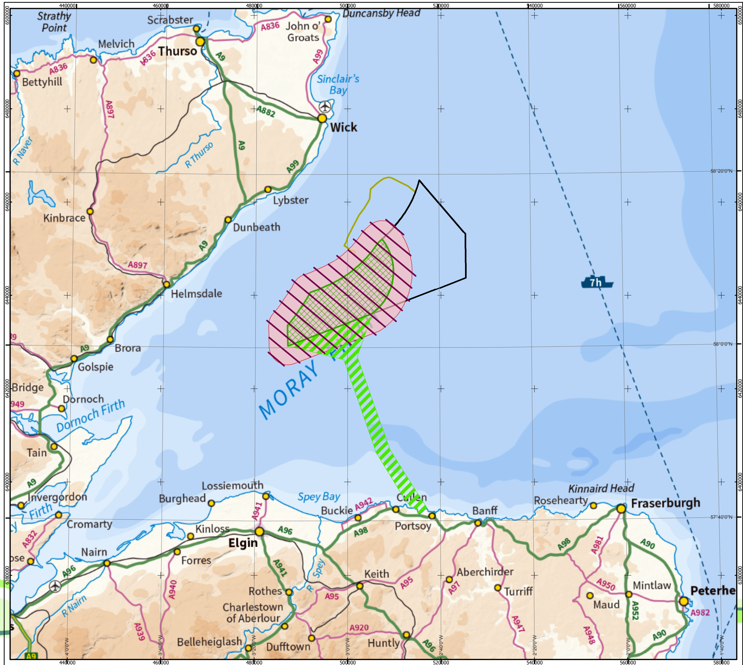
Figure 10.5.1: Moray West Aerial Surveys
