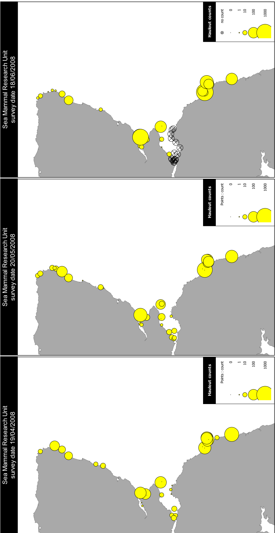
Figure 6. Monthly aerial survey counts in April-September 2008.
