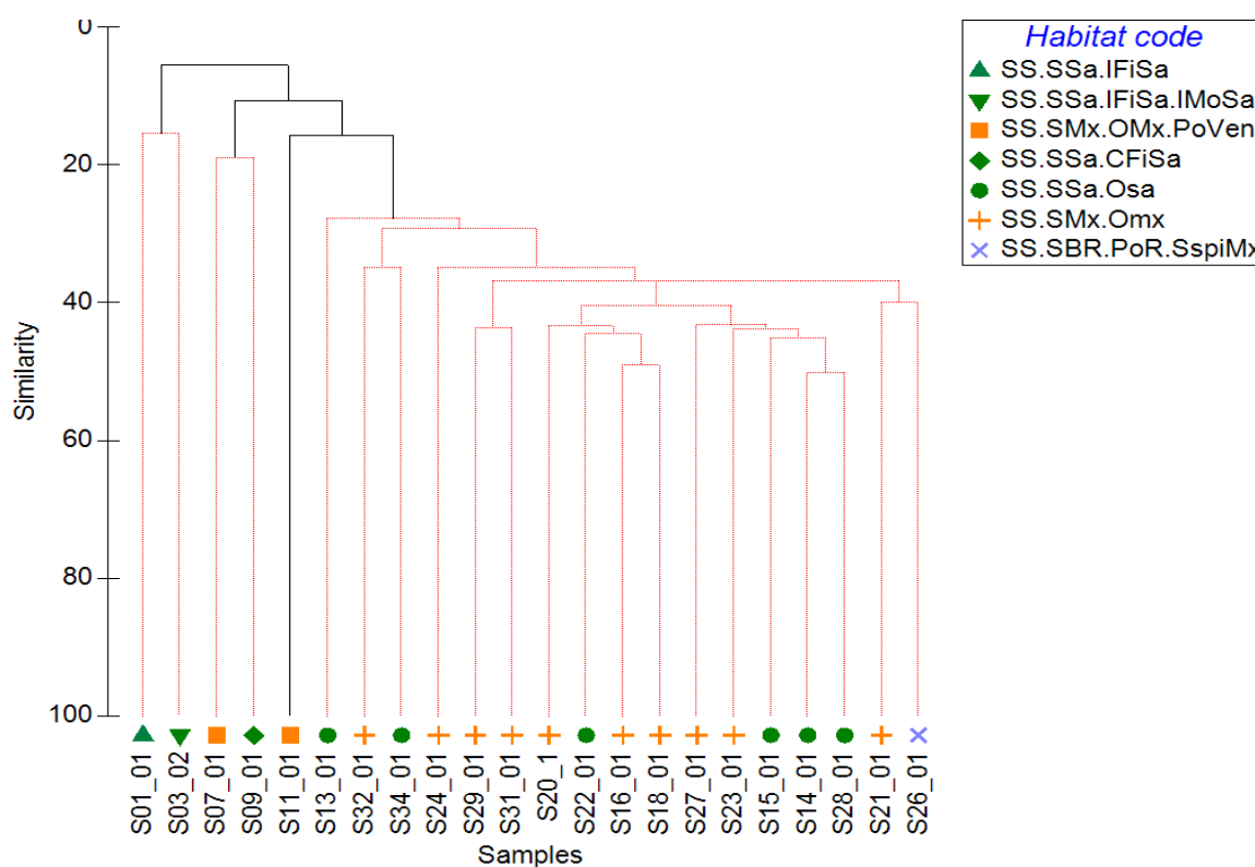
Figure 35 Dendrogram for hierarchical clustering of the 22 sites (Using group-average linking of Bray-Curtis similarities calculated on square root transformed abundance data. The JNCC habitat classifications are shown with symbols.)
