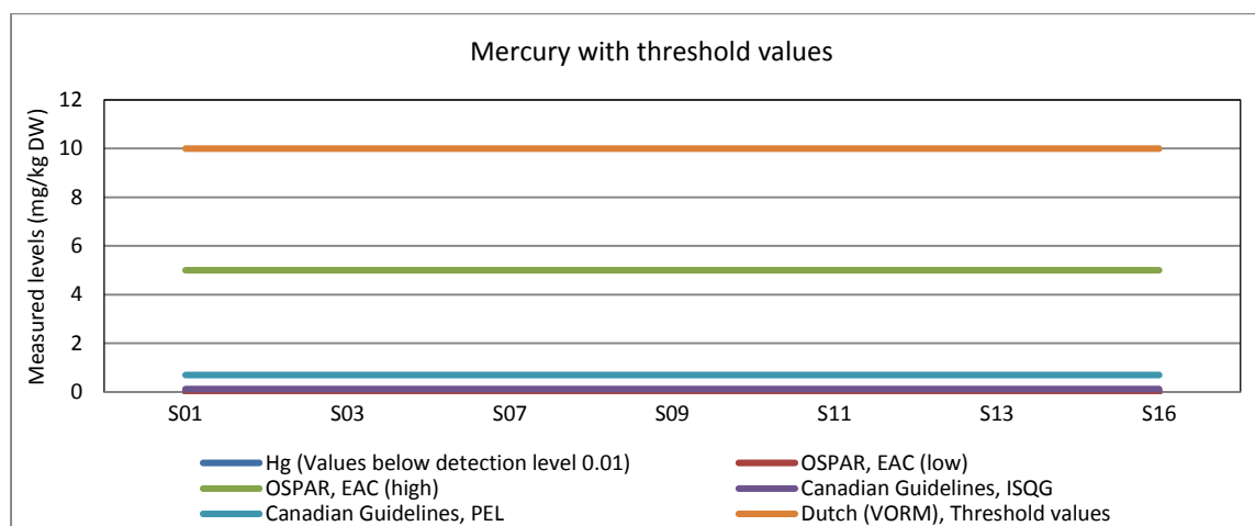
Figure 24 Mercury (Hg) concentrations with threshold values within surveyed area
