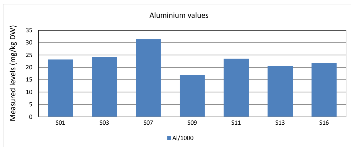
Figure 20 Aluminium (Al) concentrations within surveyed area. All values are divided with 1000.
