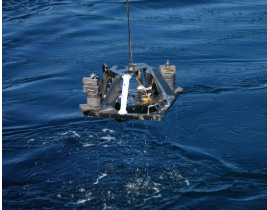
Figure 7 Day Grab sampler
