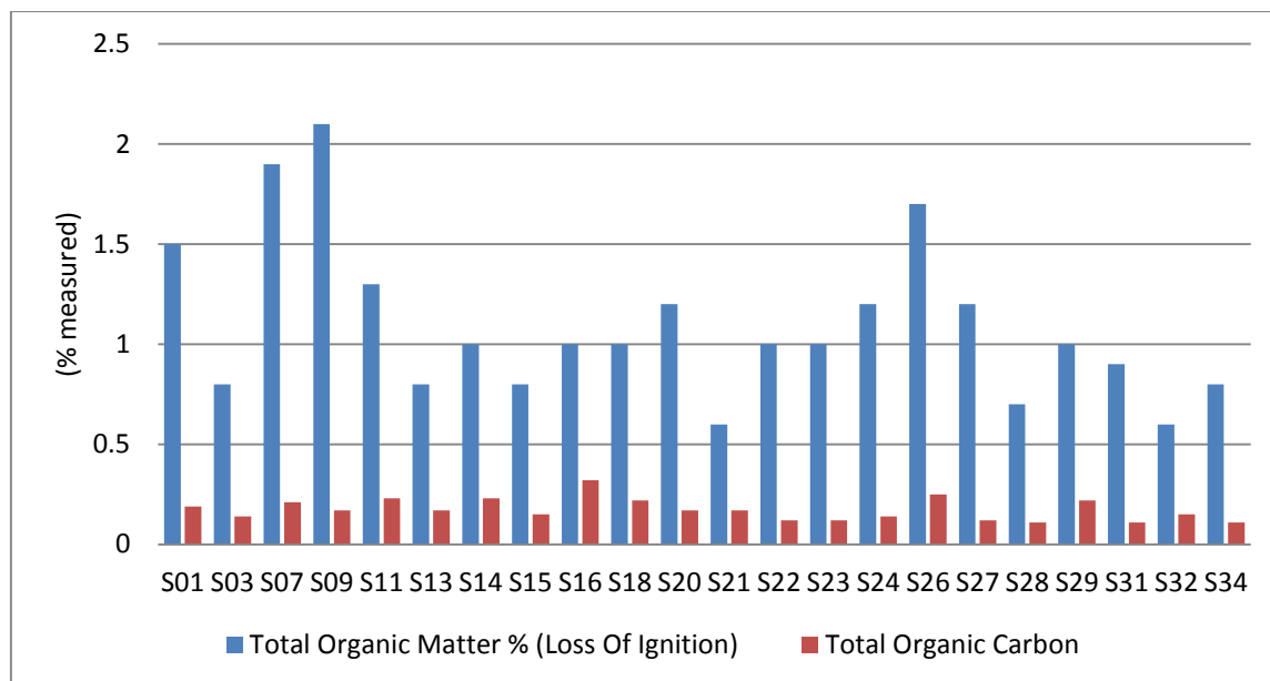
Figure 30 Summary of the total organic matter and carbon within the surveyed areas.
