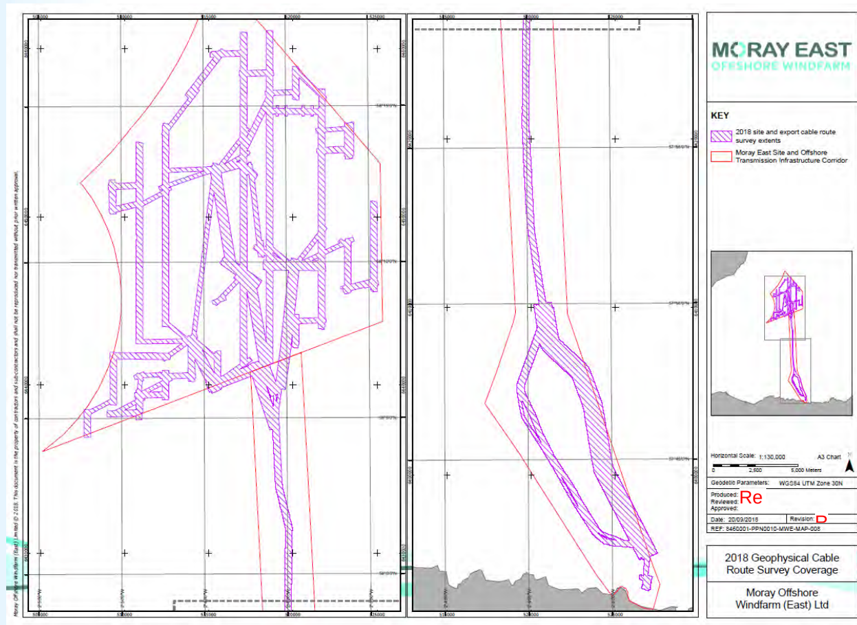
Figure 8-2: Geophysical Coverage 2018.
