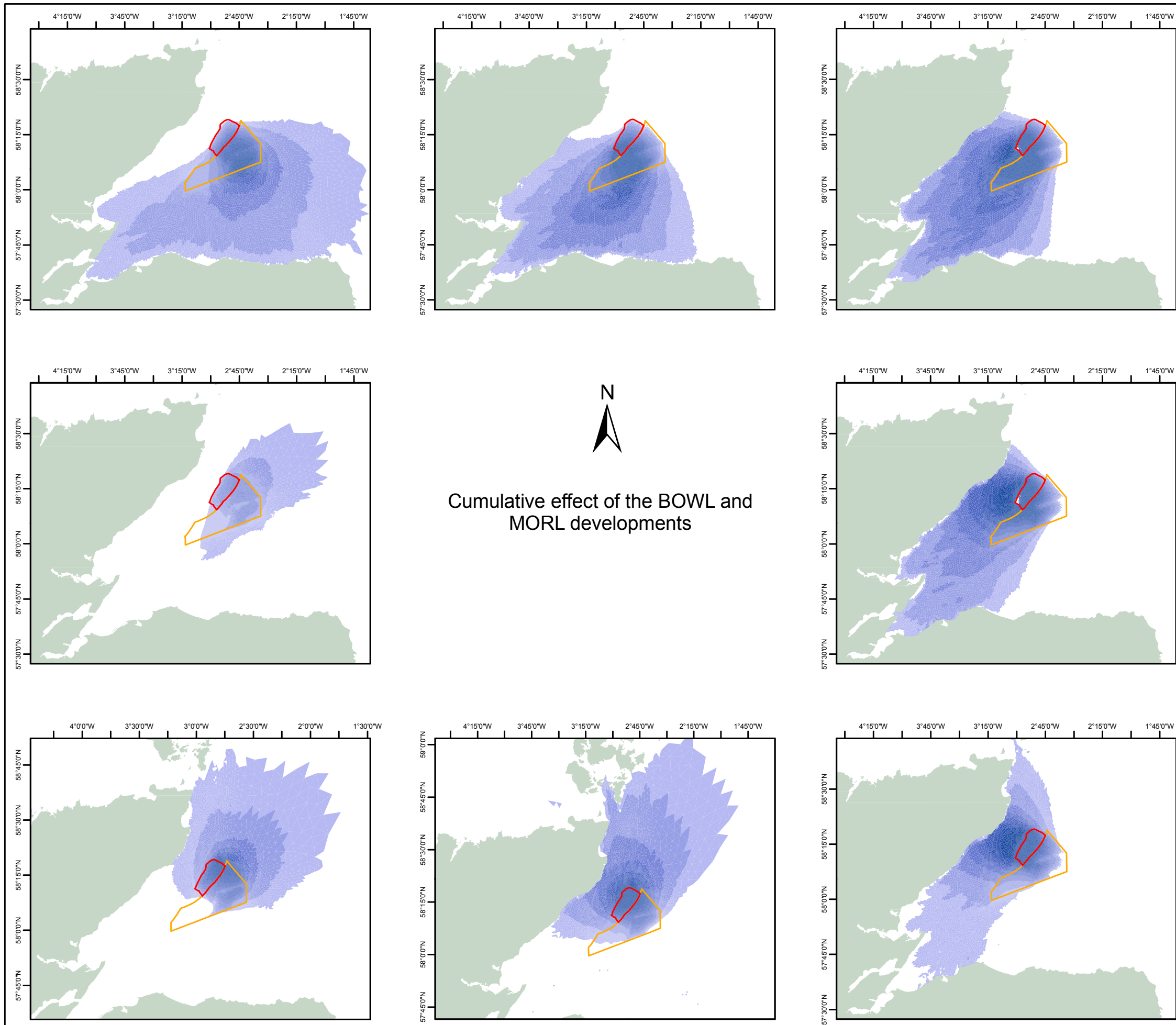
UK Offshore Development Figure 9.17 Combined Effect of the BOWL and MORL Developments on Wave Height (GBS, 1:10 Year Return Period)
