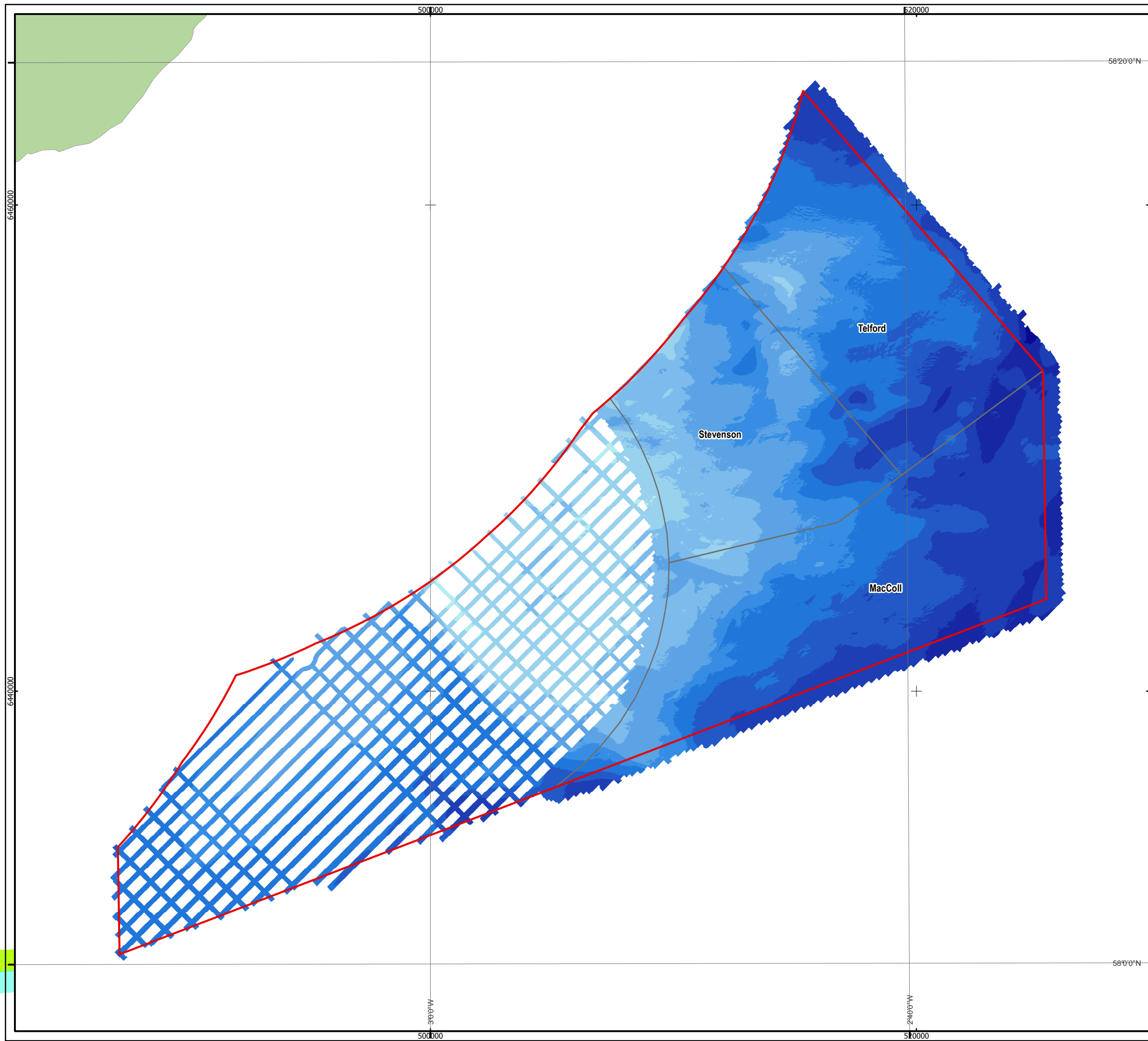
Fig 3.1-2 - Swathe Bathymetry of the Project Area
