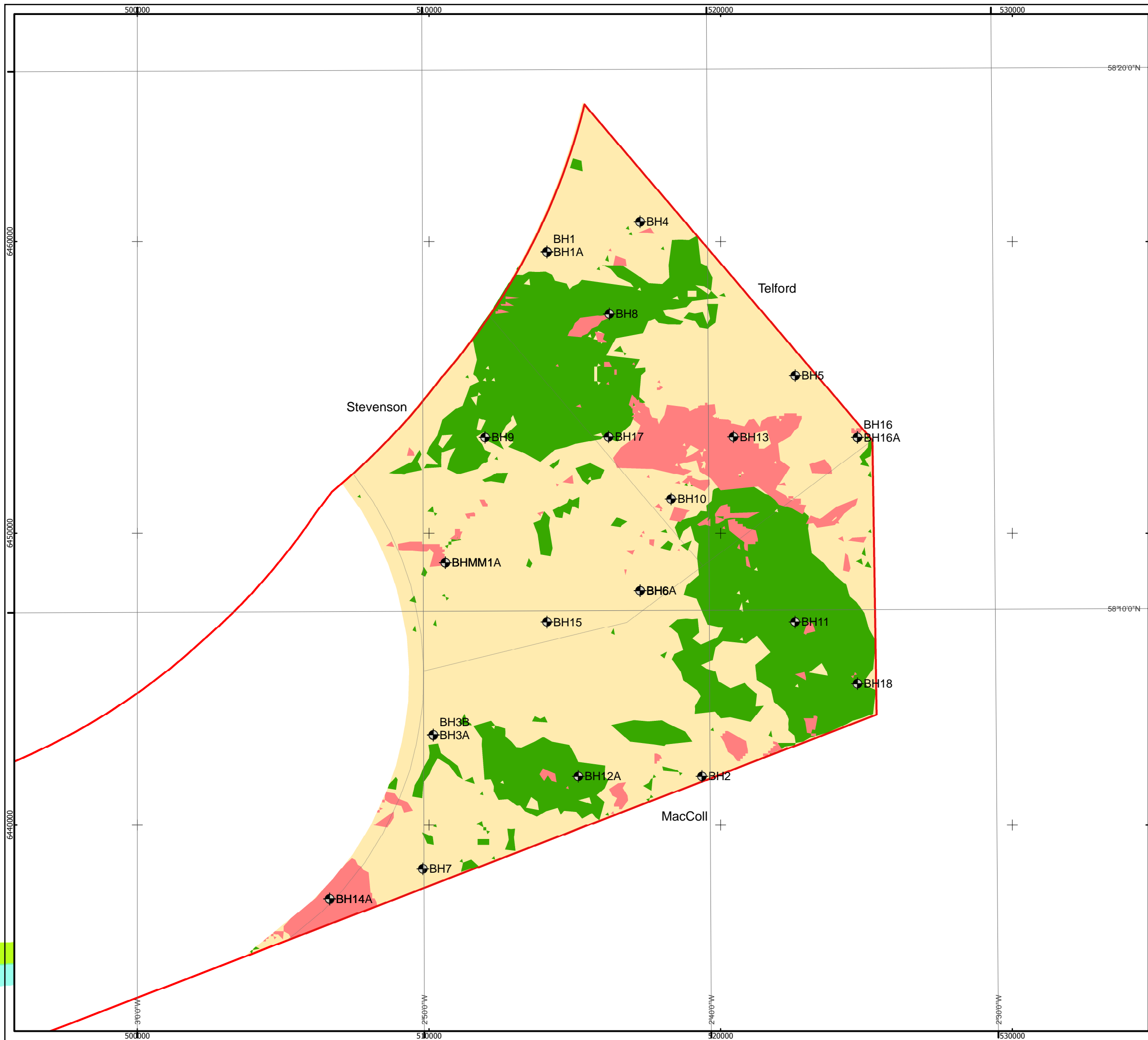
Fig 3.6-2 Soil Province Map & Borehole Locations
