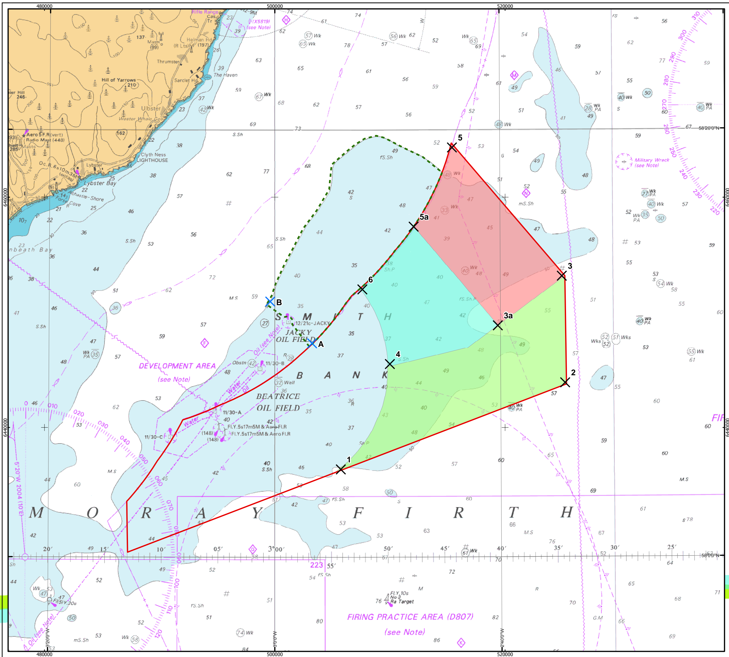
Fig 3.6-3 Locations of modelled pile driving activity for cumulative noise impact studies
