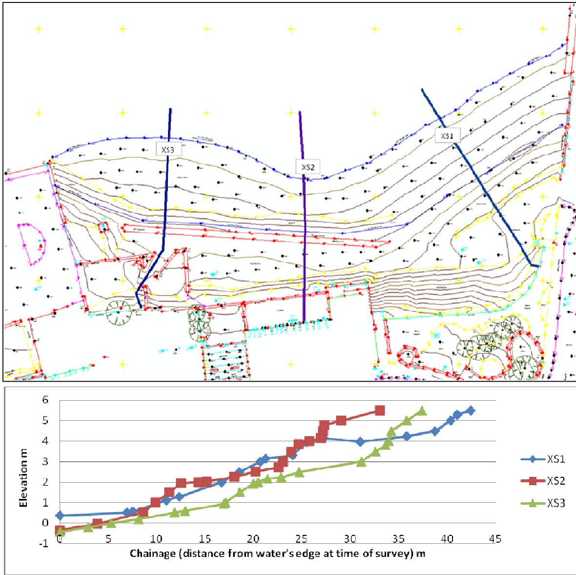
Figure 2: Cross-sections of the site, extracted from topographic survey
