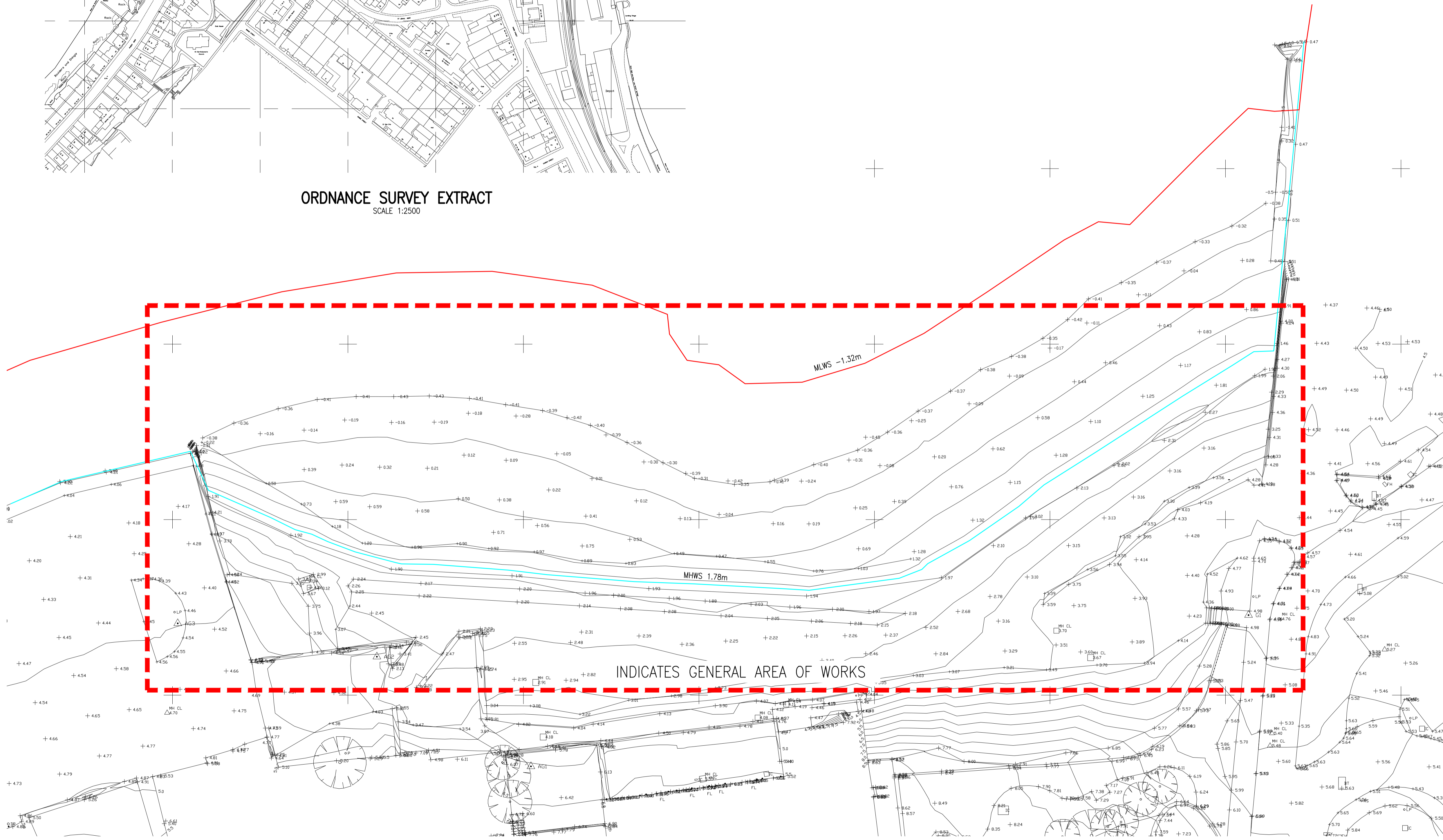
TOPOGRAPHICAL SURVEY SCALE 1:250
