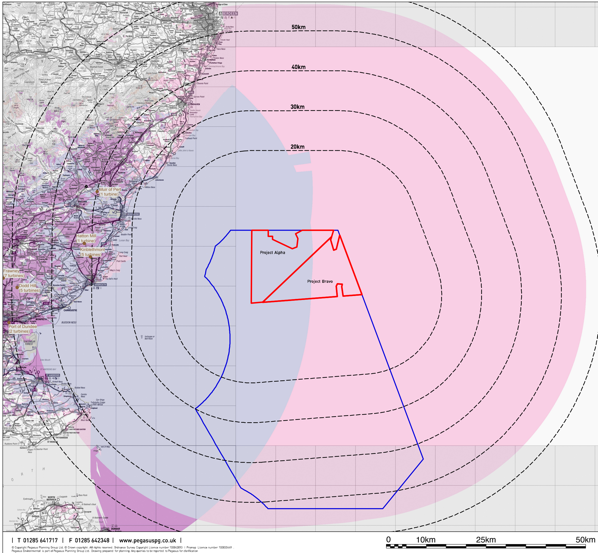
Fig 16.40 Seagreen Project with Scoping Onshore Wind Farms ZTV
