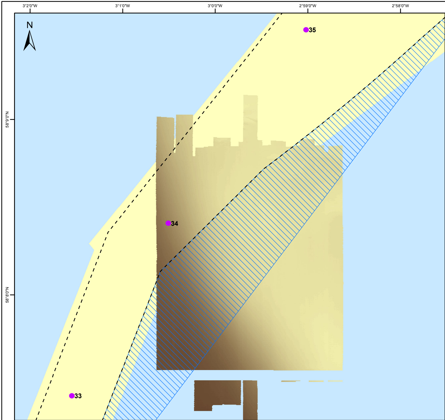
UK Offshore Development Figure 10.1 Sea Bed Sediment Type for Amendment to Original OTW Corridor with Benthic Survey Sites from 2011
