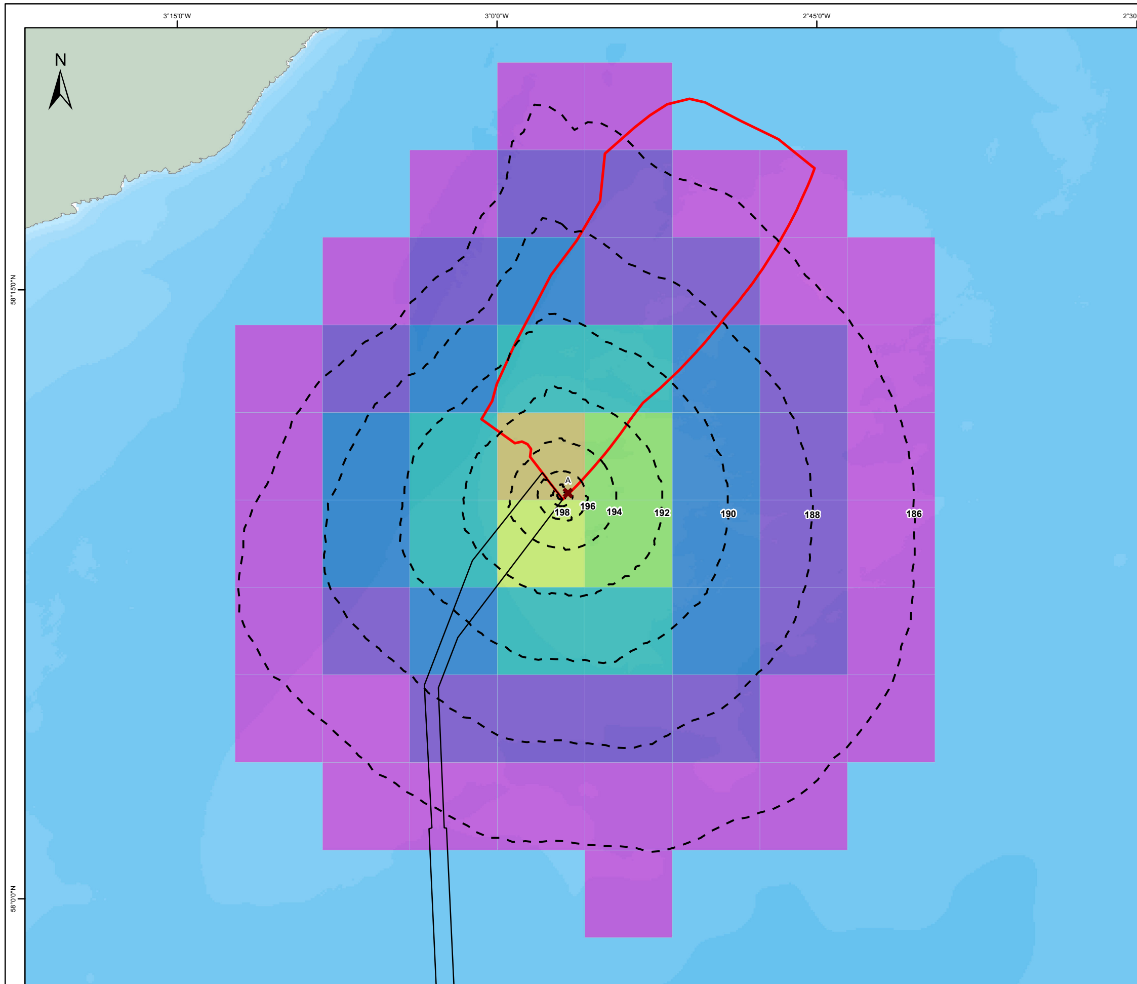
UK Offshore Development Figure 6.1 Area of Permanent Threshold Shift (PTS) for Bottlenose Dolphin for BOWL A
