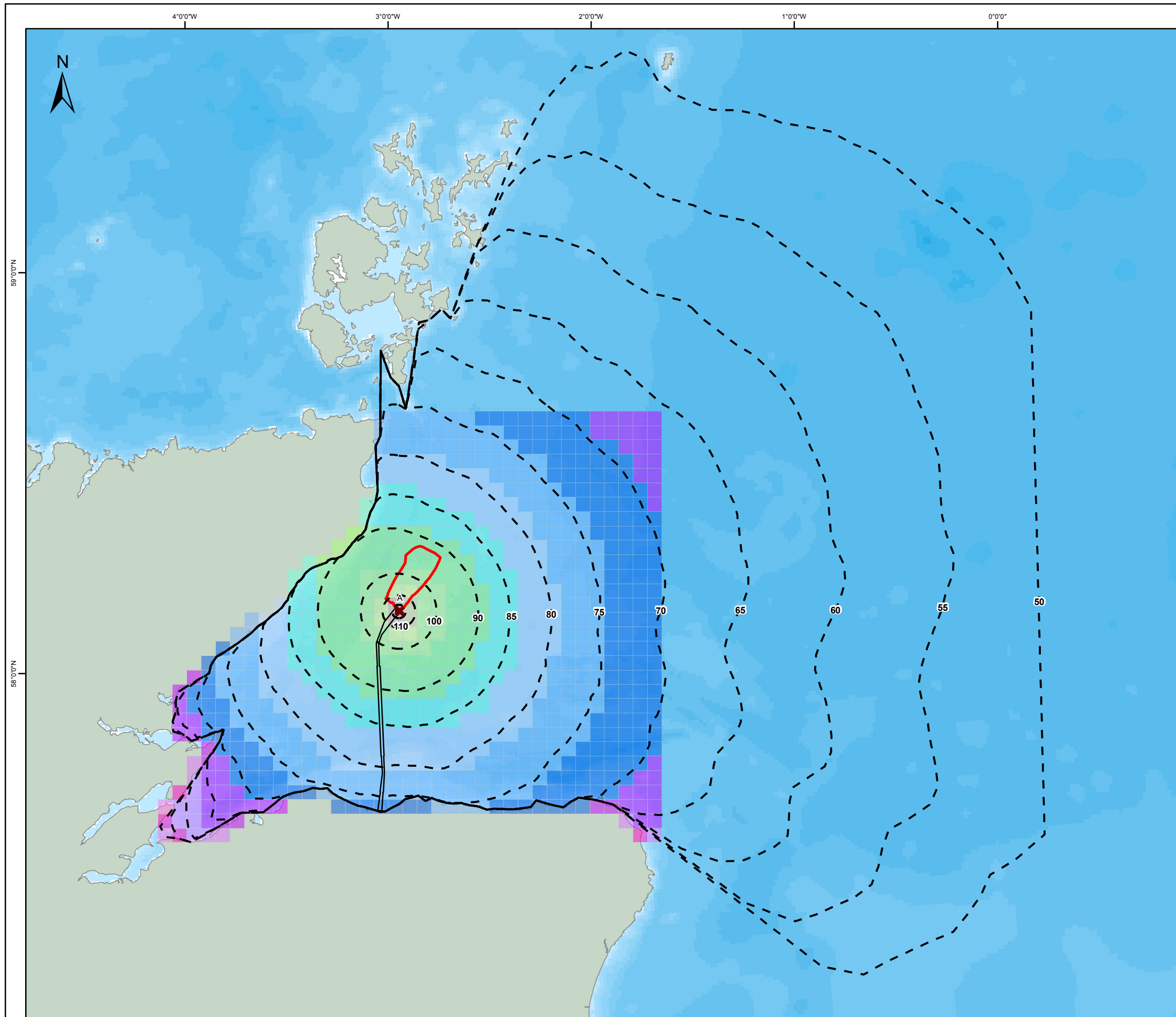
UK Offshore Development Figure 6.3 Area of Behavioural Effect (dB (HT) ) for Harbour Porpoise for BOWL A
