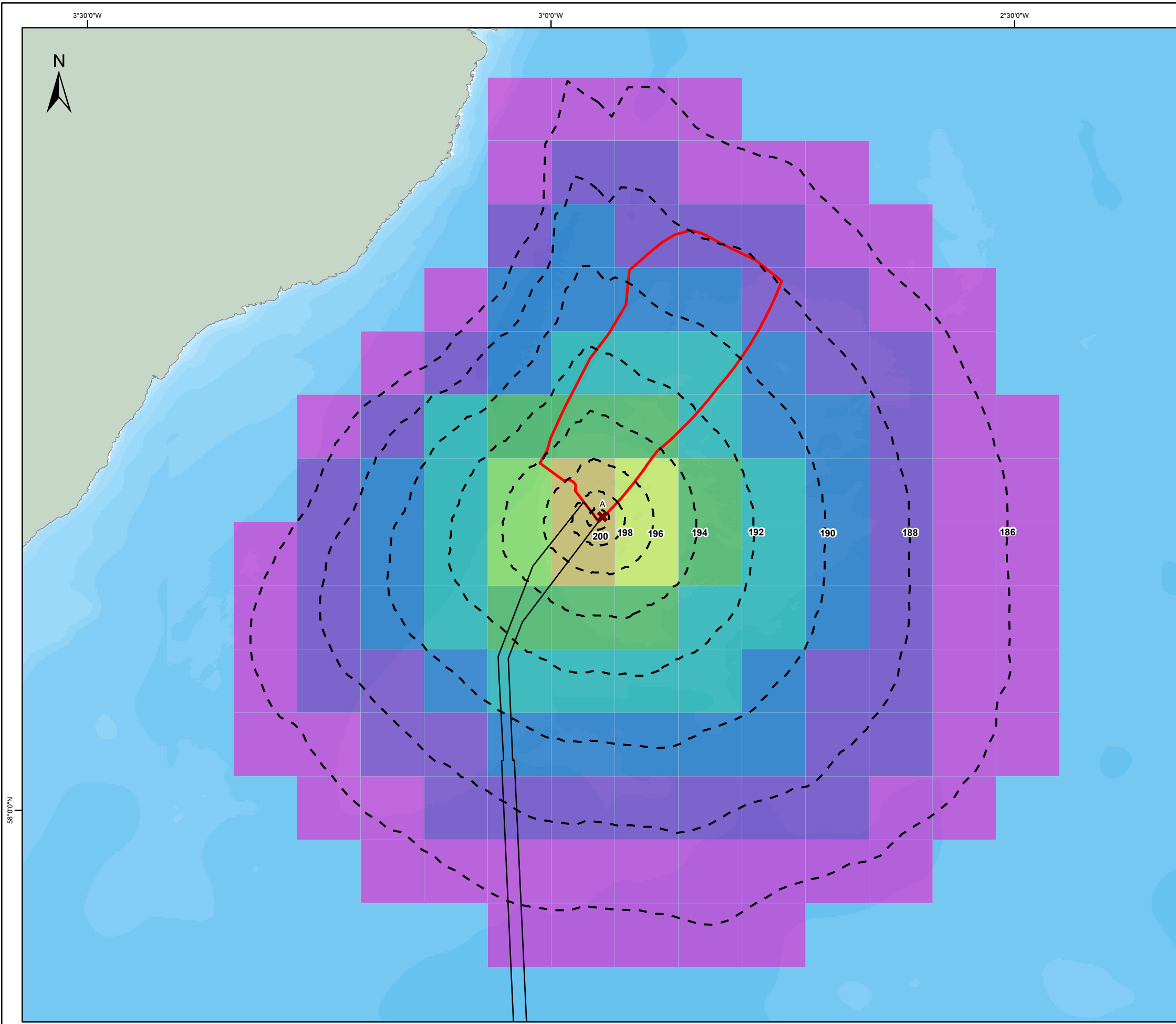
UK Offshore Development Figure 6.4 Area of Permanent Threshold Shift (PTS) for Minke Whale for BOWL A
