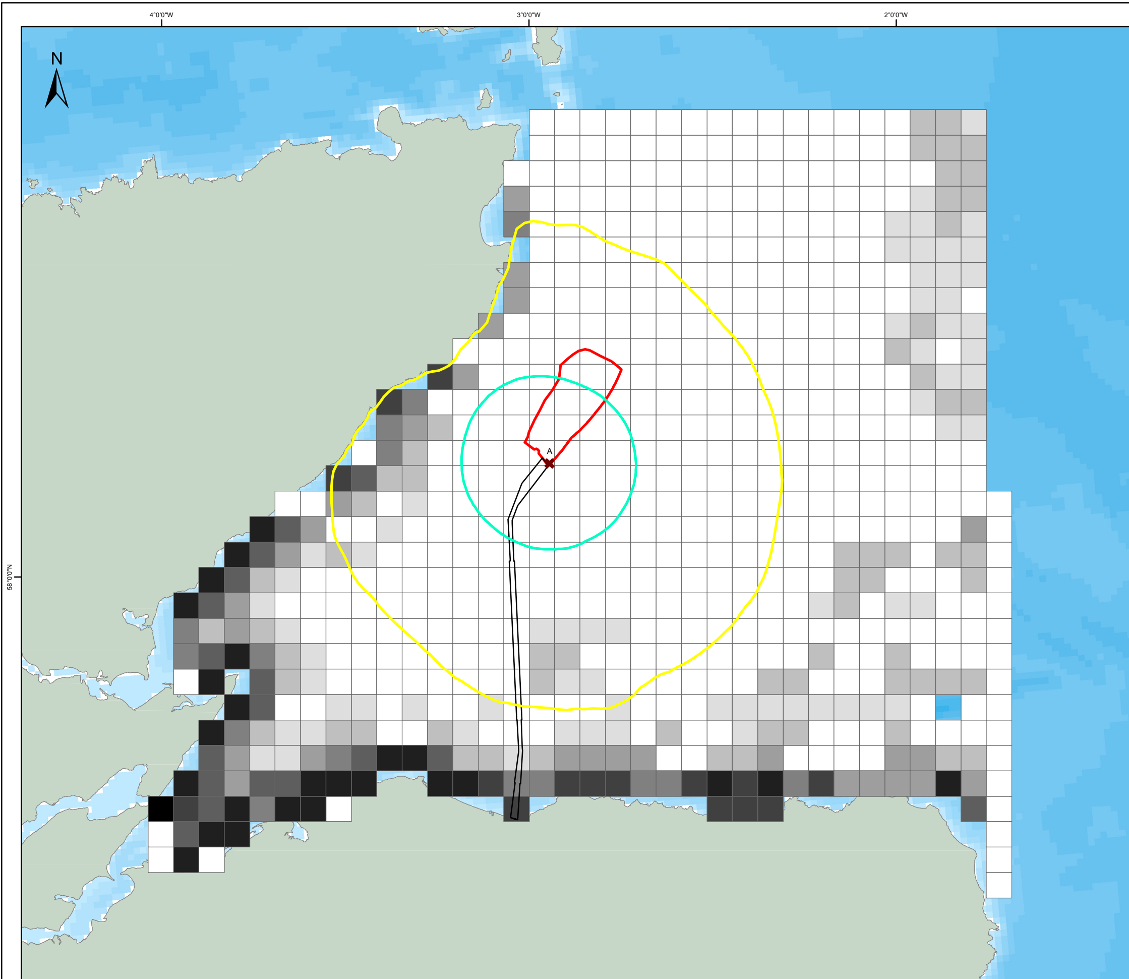
UK Offshore Development Figure 6.8 Area of Behavioural Effect (dB HT ) for Bottlenose Dolphin Using the 1800 kJ Hammer Energy
