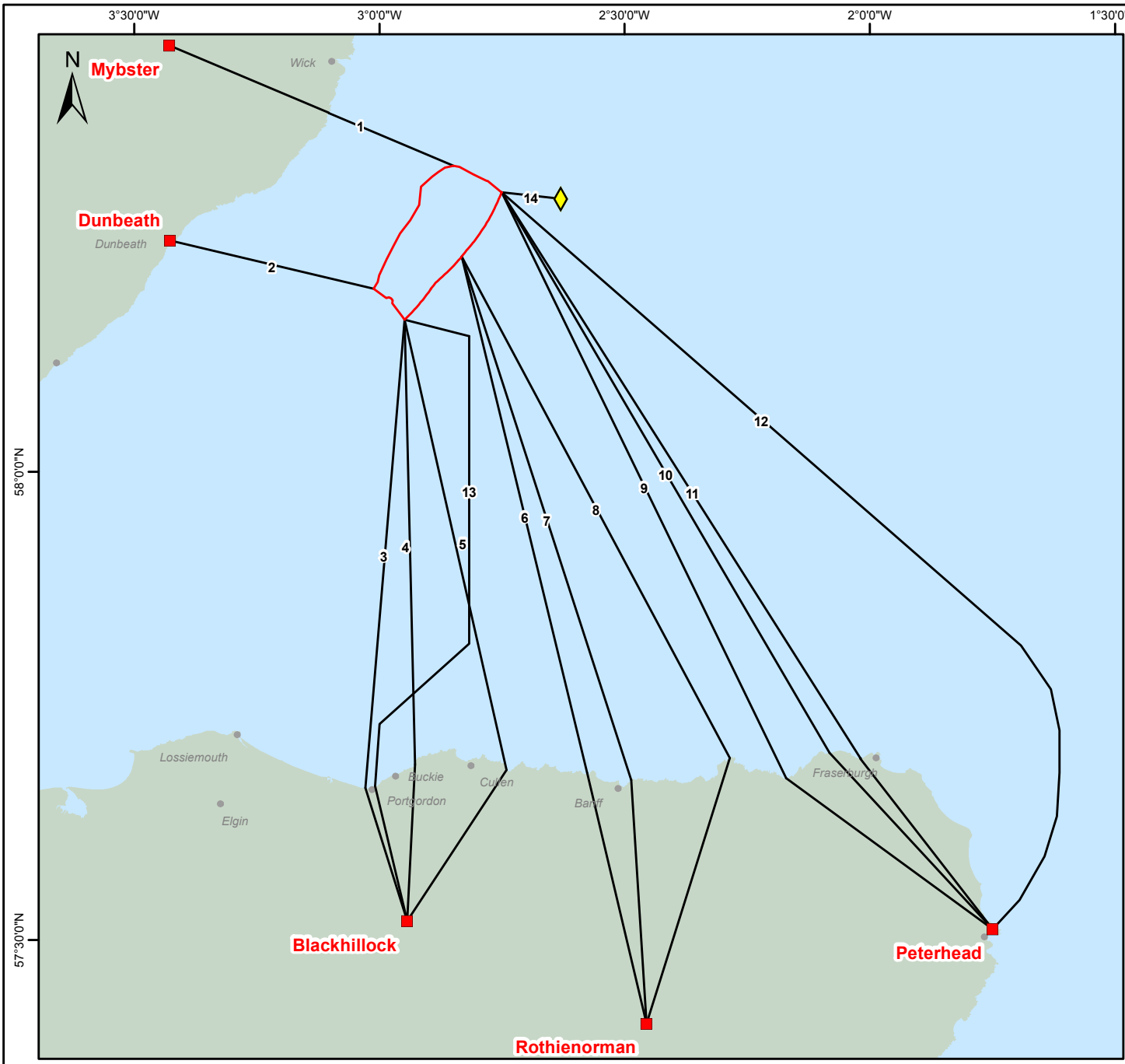
UK Offshore Development Figure 6.2 Grid Connection Point Options and 14 Offshore Transmission Works Route Options
