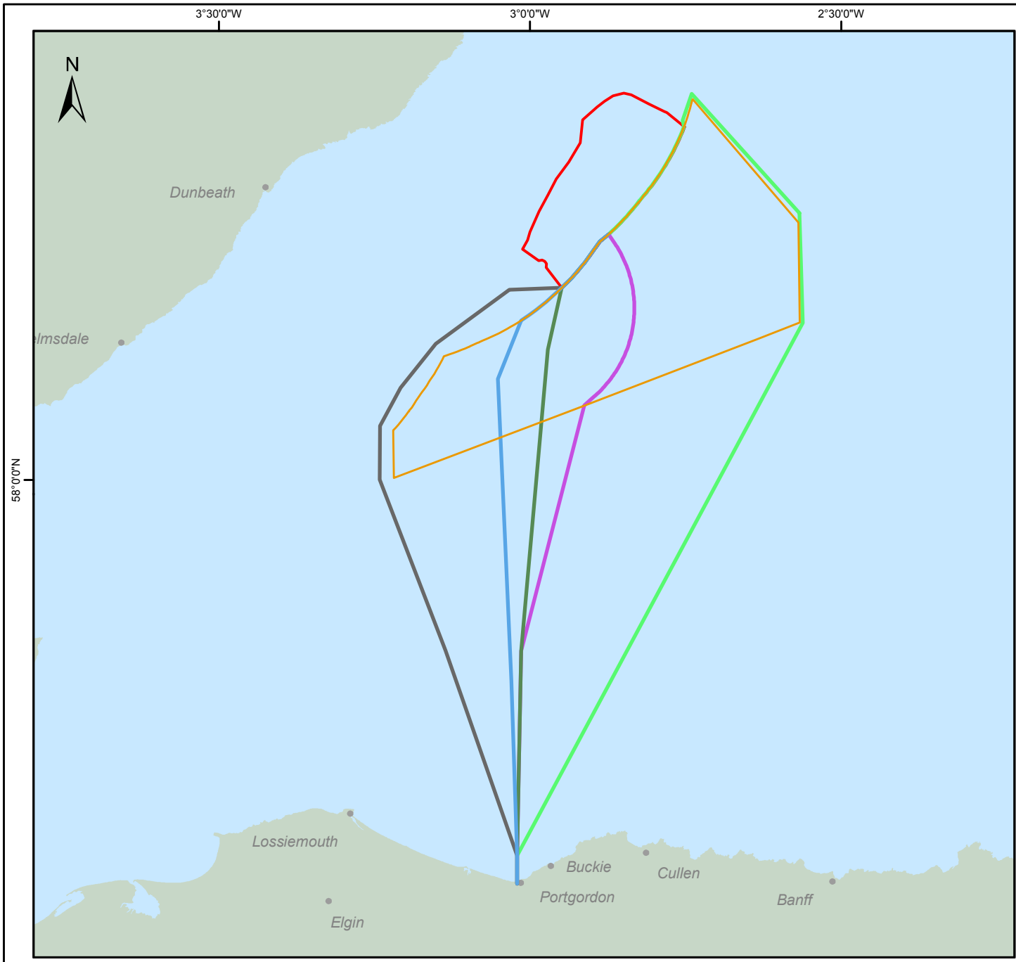
UK Offshore Development Figure 6.4 Offshore Transmission Works Route Options
