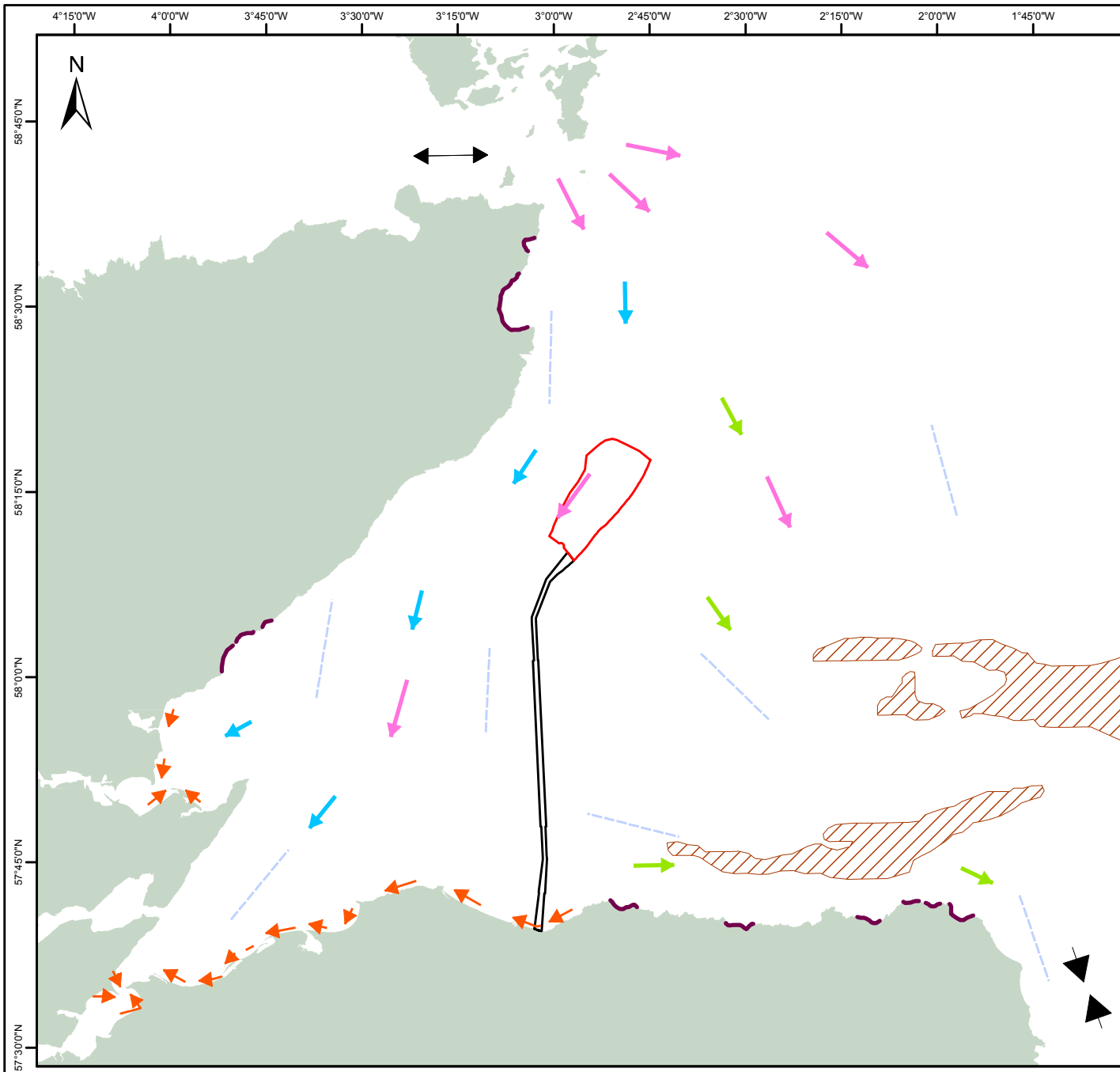
UK Offshore Development Figure 9.6 Bedload and Longshore Sediment Transport in the Moray Firth
