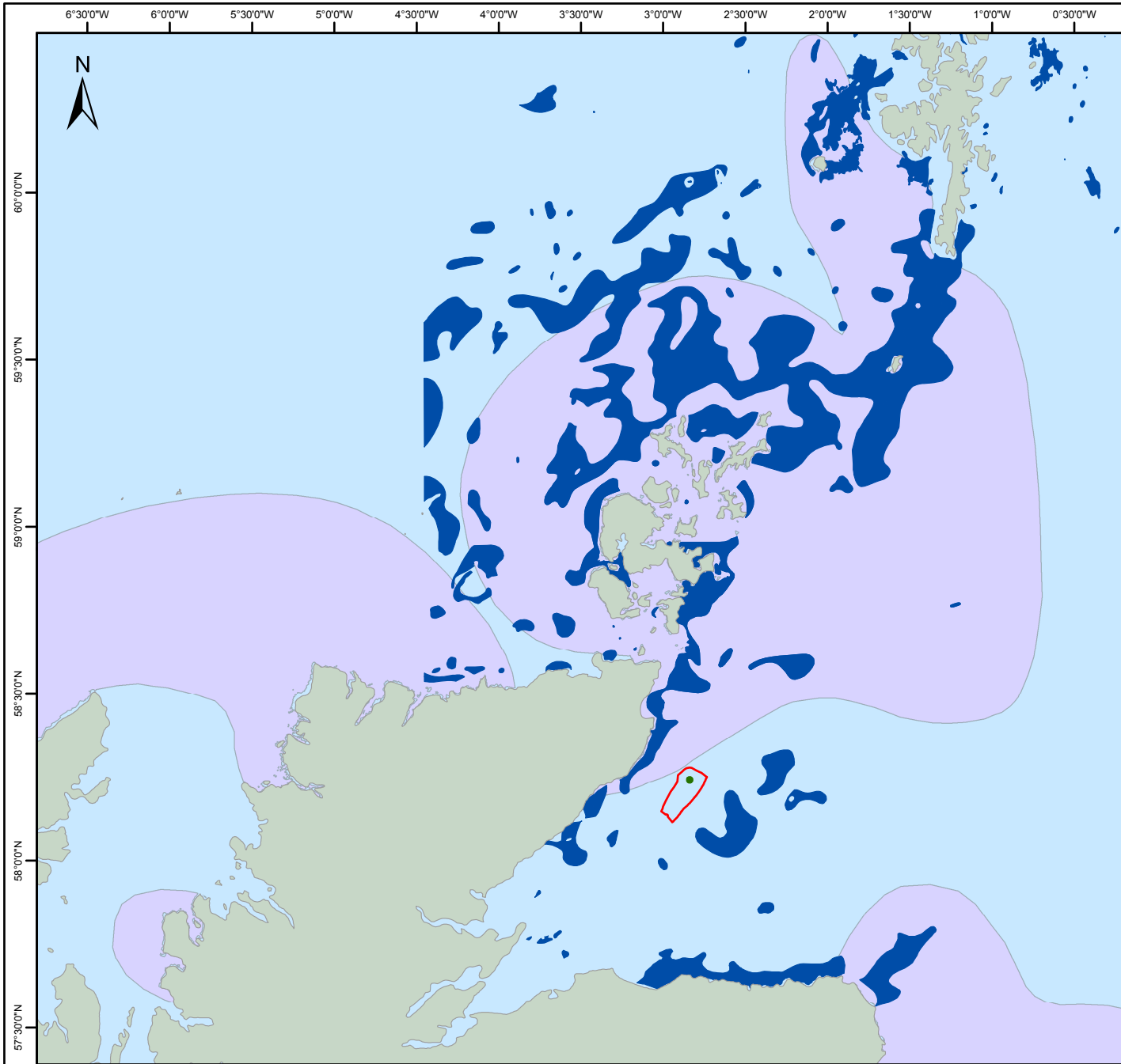
UK Offshore Development Figure 11.8 Worst Case Loss of Habitat with Gravel and Sandy-Gravel Areas and Herring Spawning Grounds (Coull et al., 1998)
