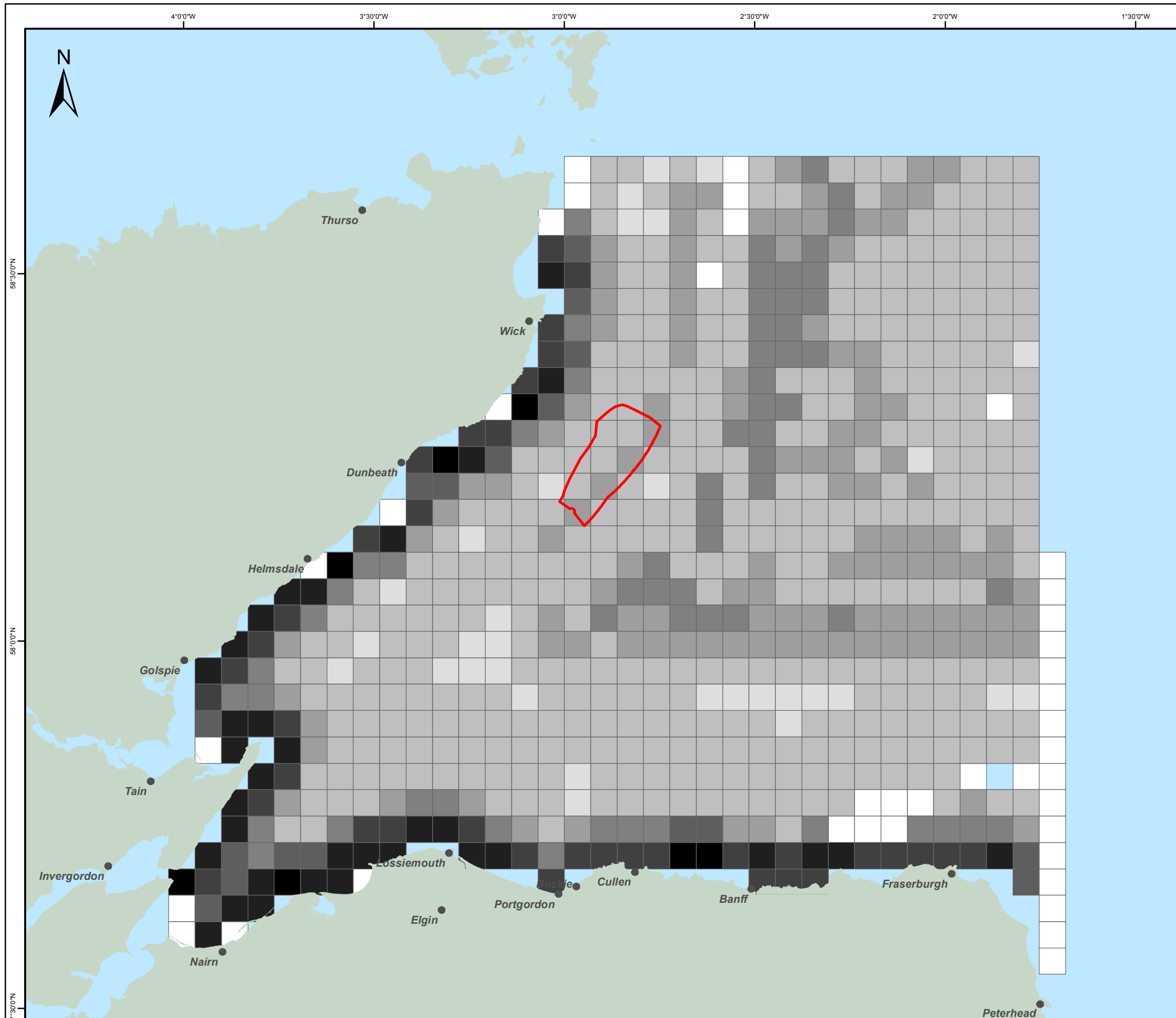
UK Offshore Development Figure 12.1 Predicted Probability of Encountering 'Dolphins' in Each 4x4 km Grid Cell Based on 2009 & 2010 Data
