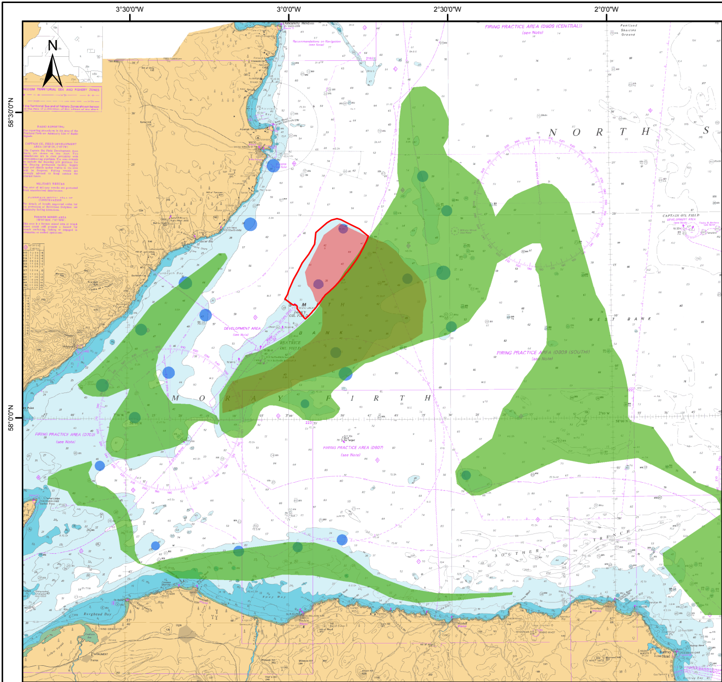
UK Offshore Development Figure 16.8 Scallop Fishing Grounds by Vessel
