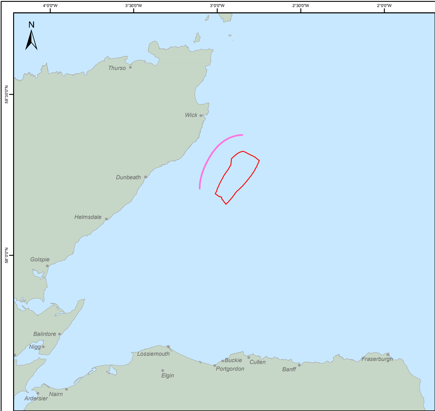
UK Offshore Development Figure 17.1 Indicative 35 dB LA90 Contour for 7 MW Scenario
