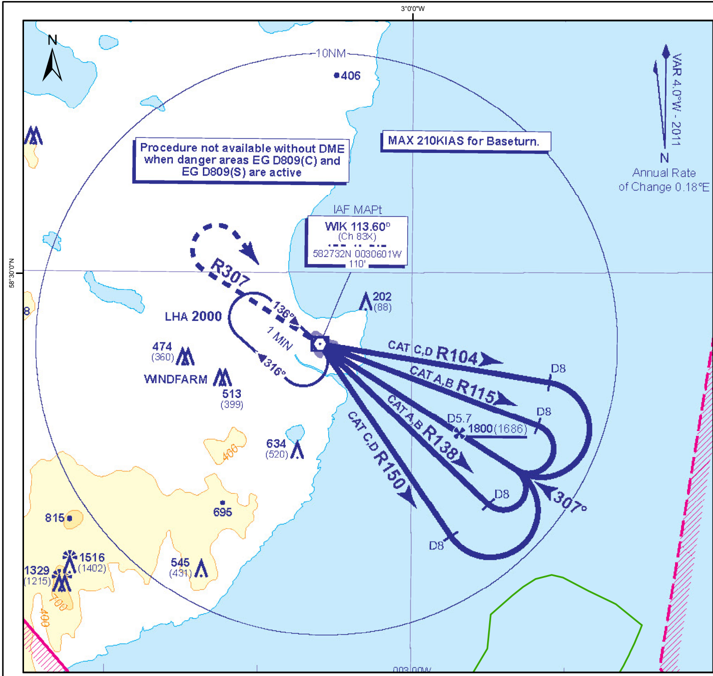
UK Offshore Development Figure 19.2 Wick VOR/DME Runway 31 Procedure
