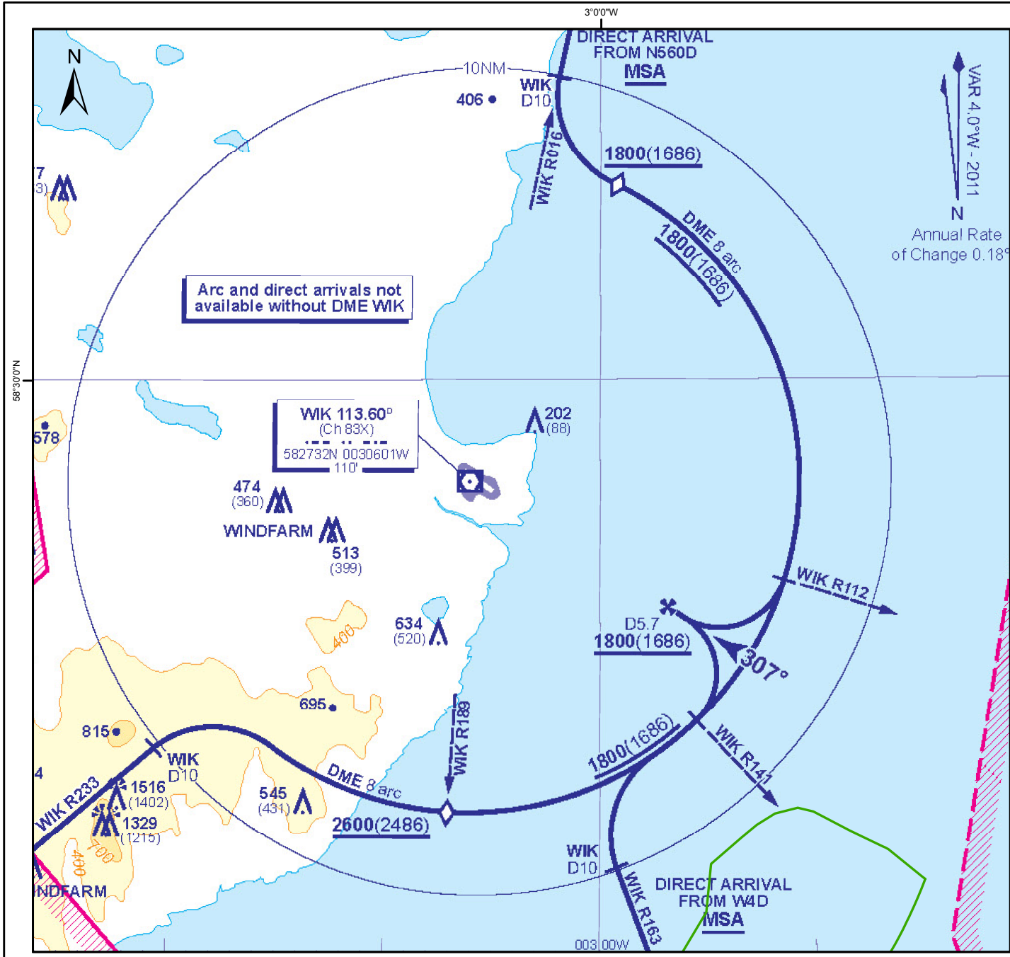
UK Offshore Development Figure 19.3 Wick Direct Arrivals to VOR/DME Runway 31 Procedure
