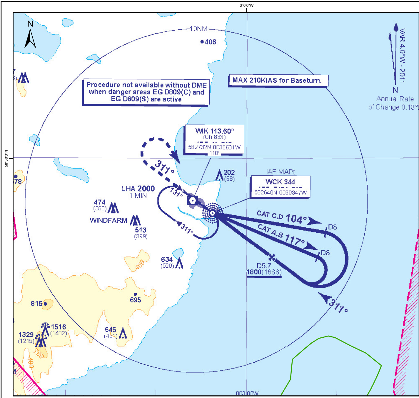
UK Offshore Development Figure 19.4 Wick NDB(L)/DME Runway 31 Procedure
