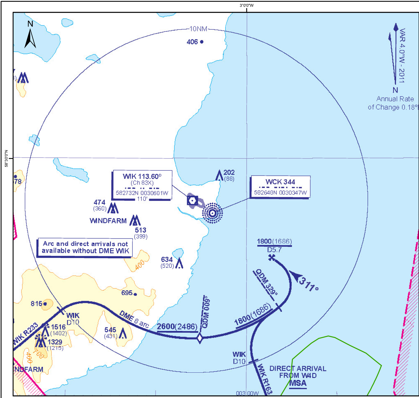
UK Offshore Development Figure 19.5 Wick Direct Arrivals to NDB(L)/DME Runway 31 Procedure
