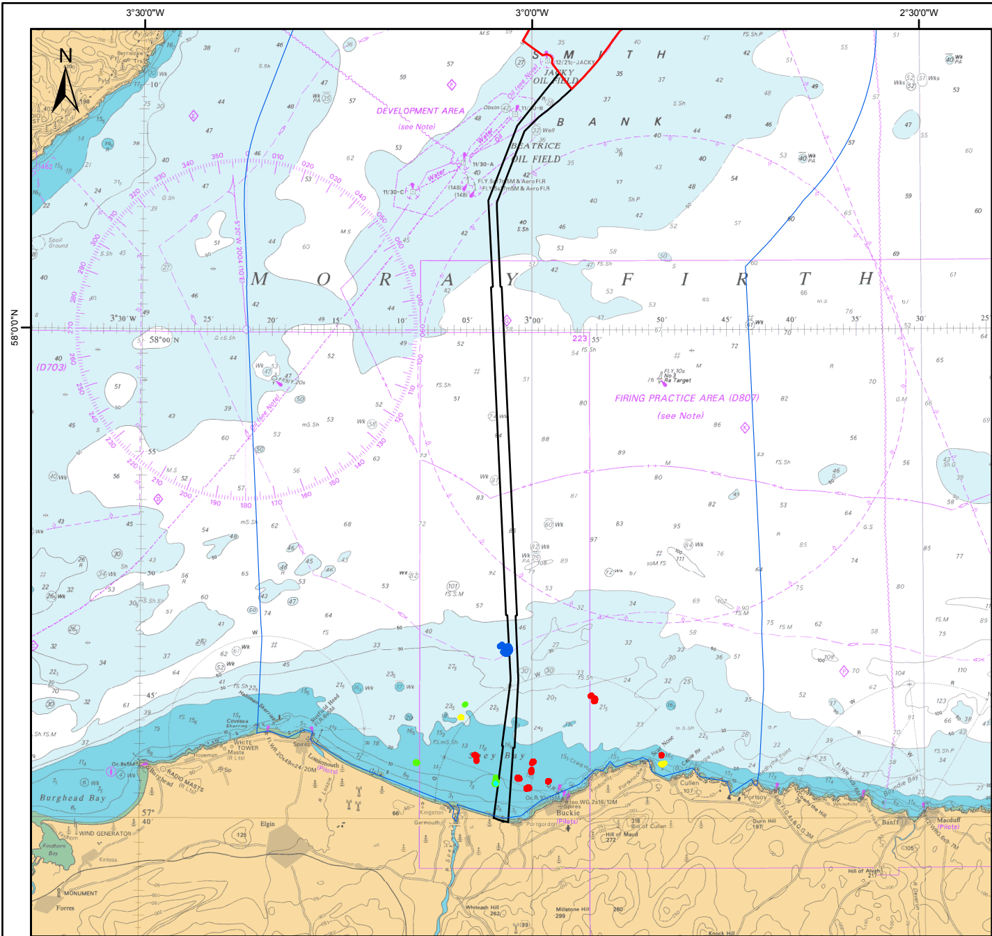
UK Offshore Development Figure 28.4 Overview Plot of Chartwell (28 days) and Gargano (28 days) Anchored Vessel Tracks within 10nm of Cable Corridor
