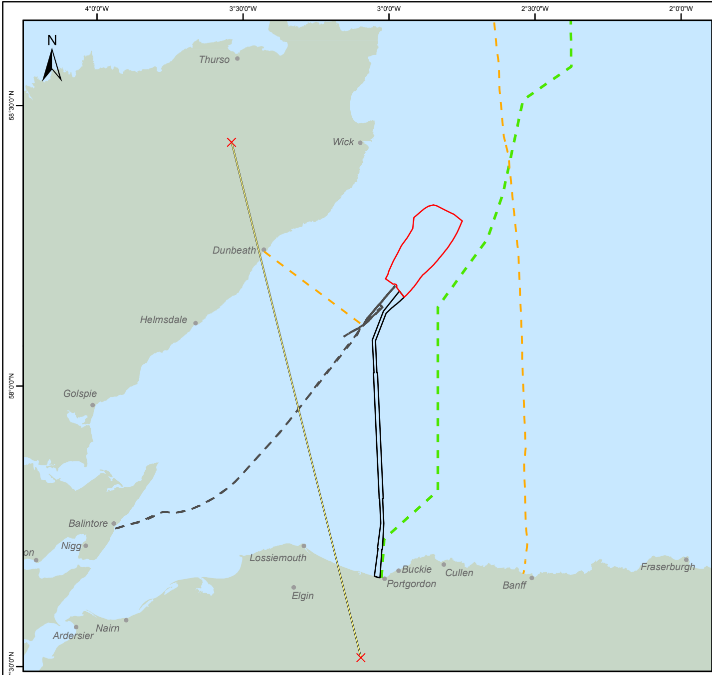
UK Offshore Development Figure 30.2 Offshore Telecommunications, Pipelines and Cables
