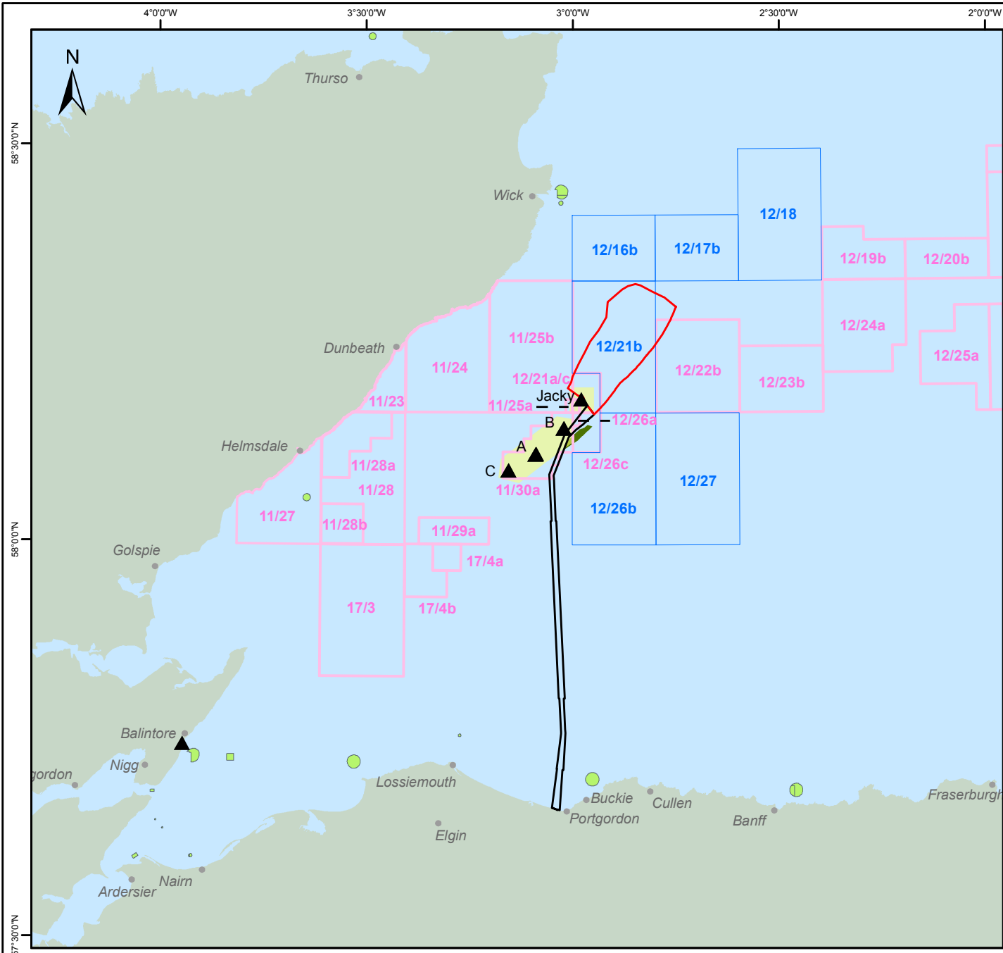
UK Offshore Development Figure 30.4 Oil and Gas Infrastructure
