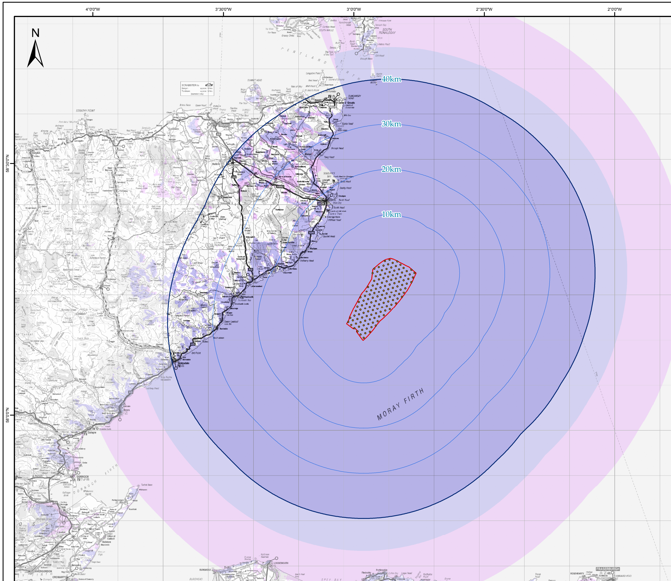
Figure 14.2 Zone of Theoretical Visibility (ZTV) - bareground
