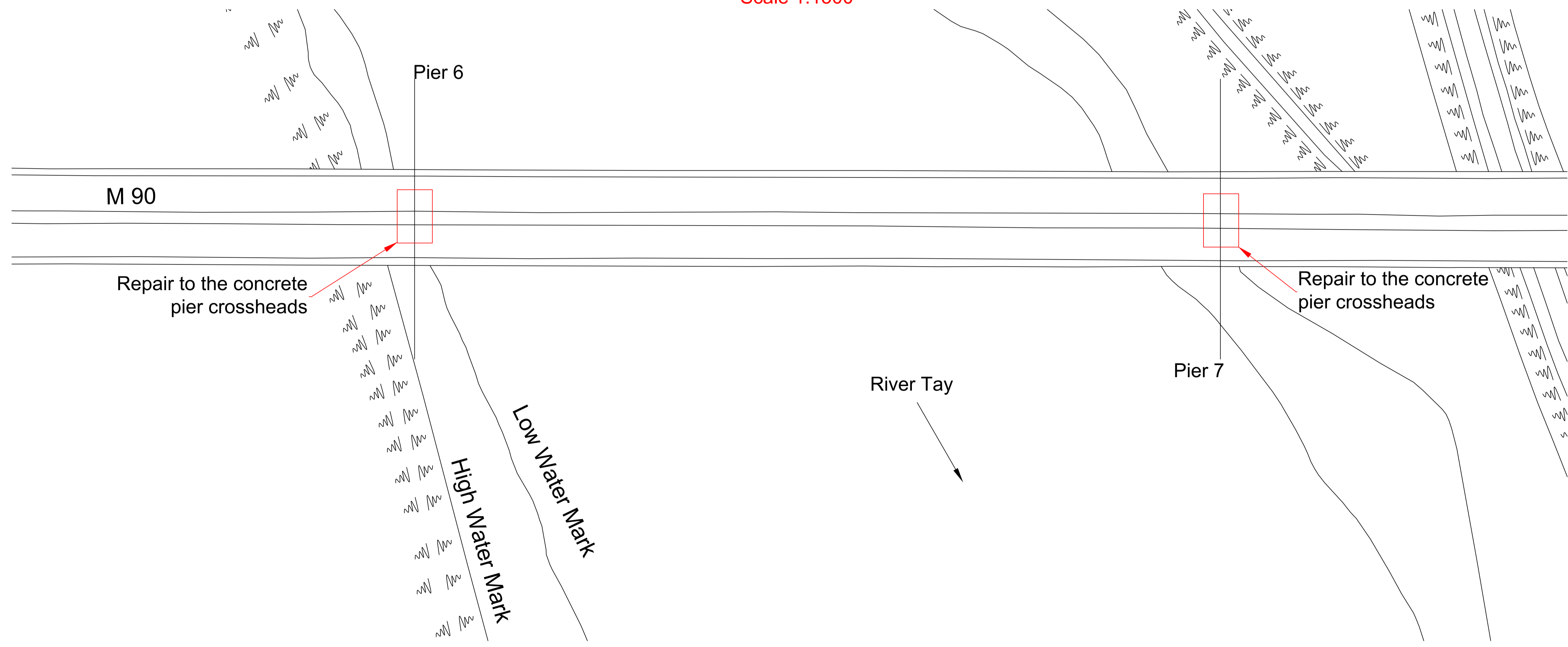
Locations of Concrete Repairs Scale 1:500
