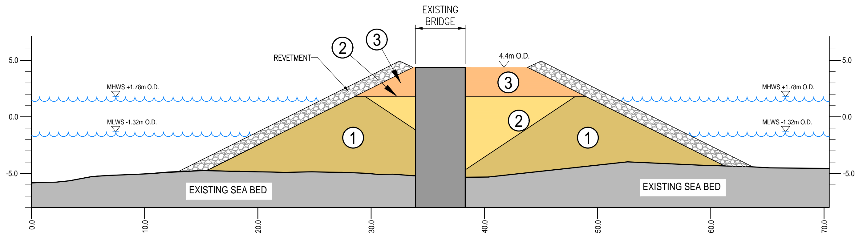
SECTION 1-1 SCALE 1:200
