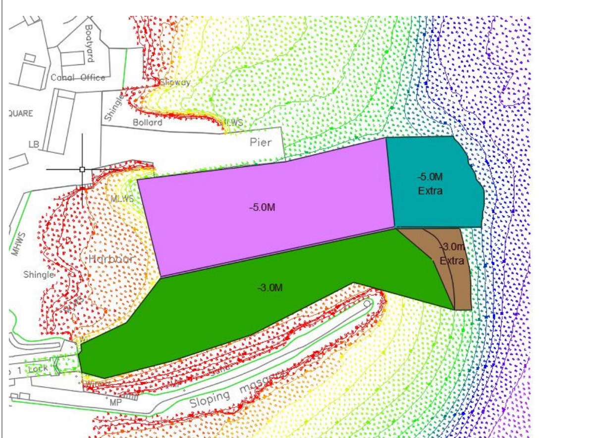
DREDGE AREAS, ARDRISHAIG HARBOUR
