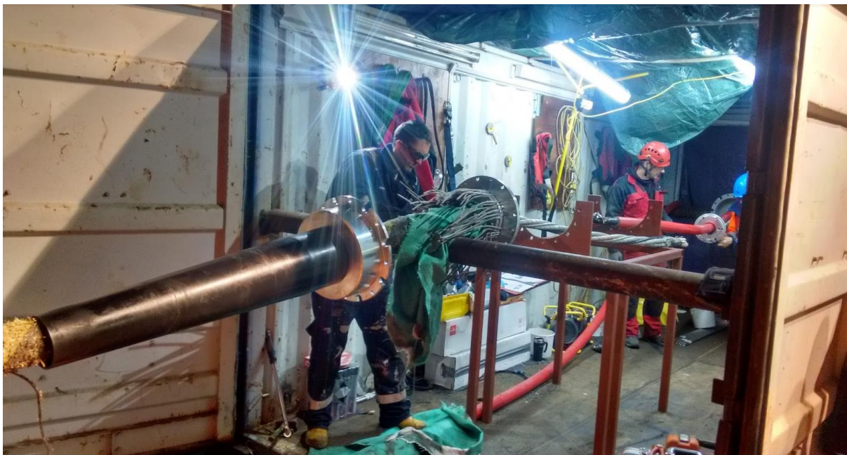
Figure 14. Orbital Marine Power and HV Contractors offshore on a multi-cat vessel cable jointing or “splicing” operations where static cables are permanently connected to the platform cable which supplies power and communications.
