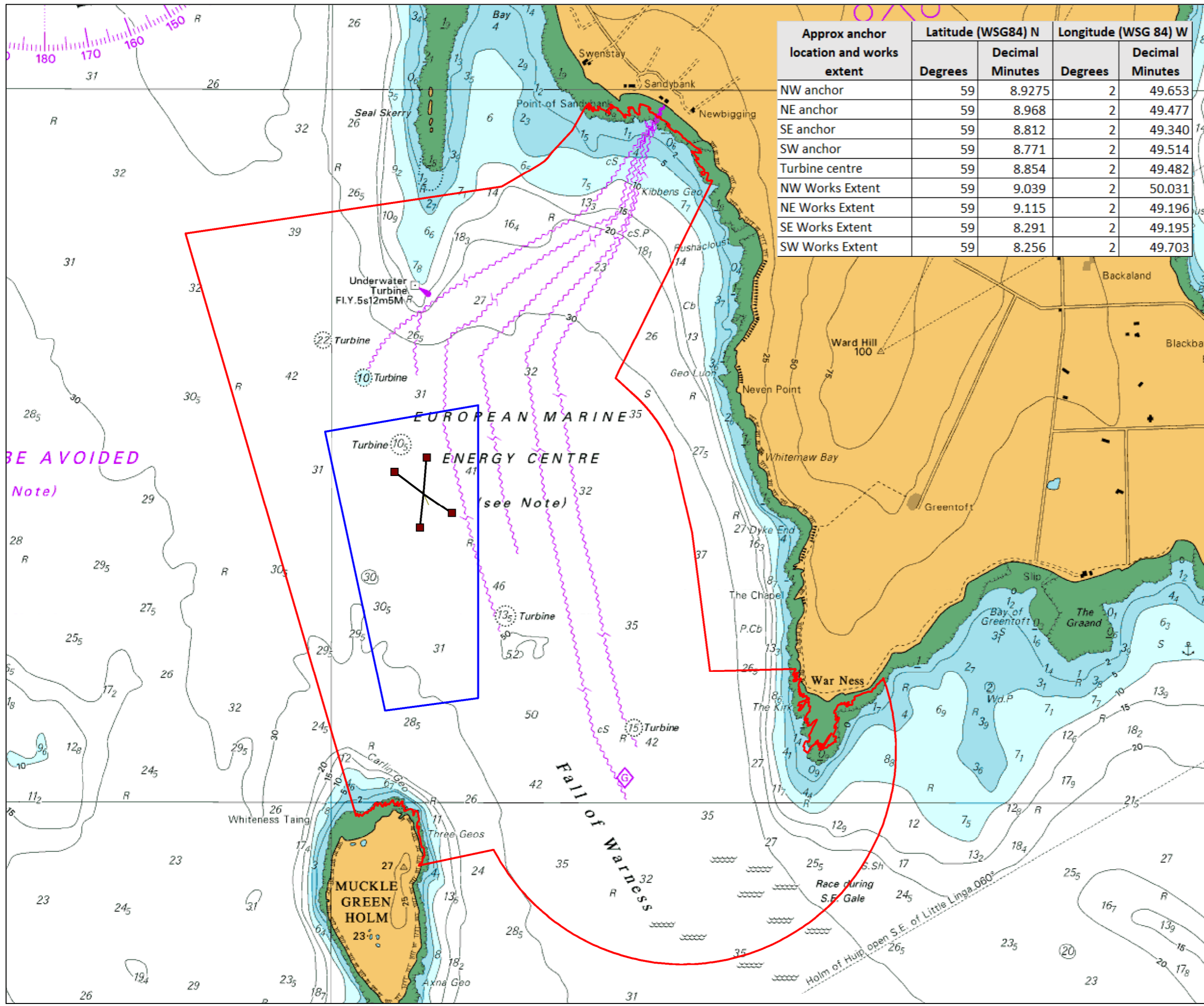
Figure 17 Site layout
