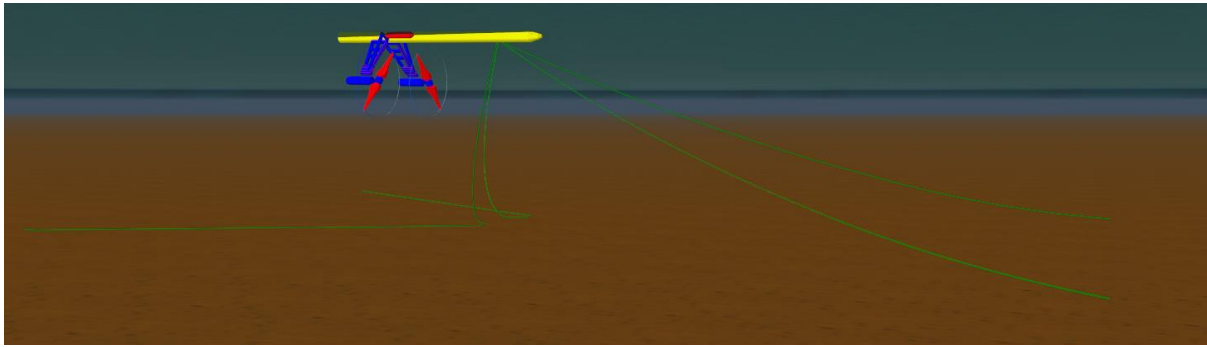
Figure 5 Orbital O2-X mooring system Composition of Mooring Lines
