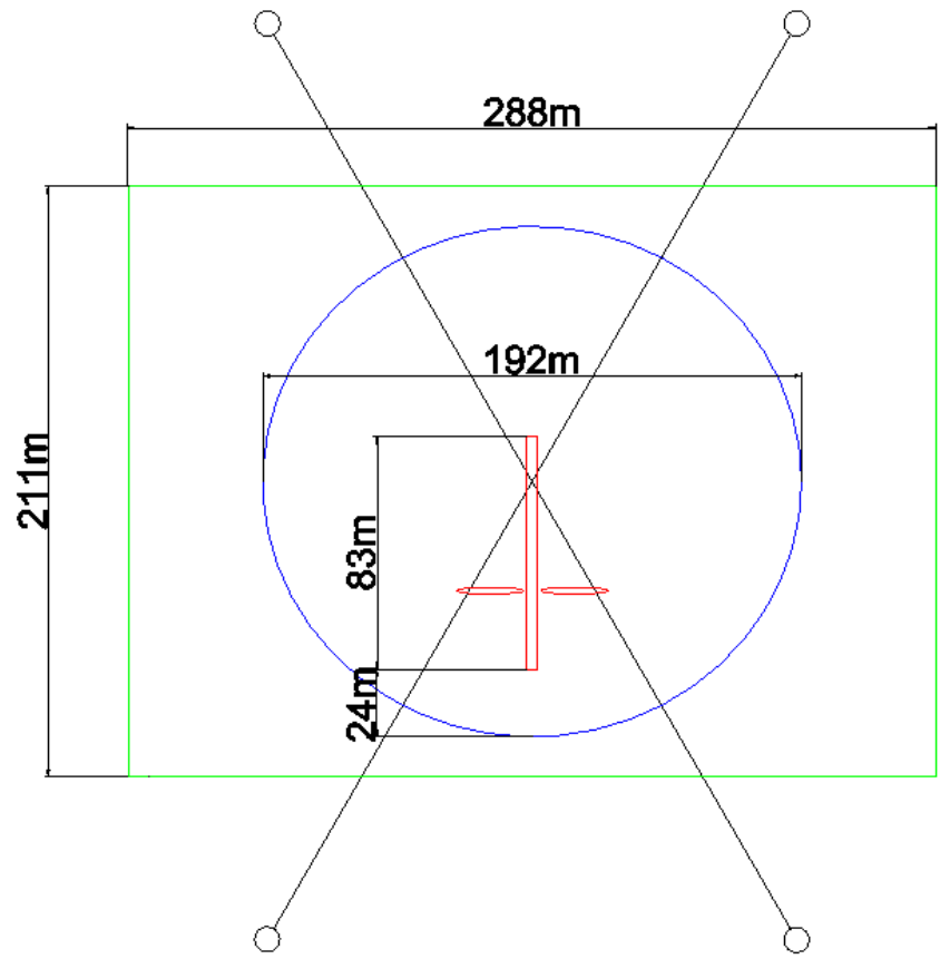
Figure 6 Mooring line schematic
