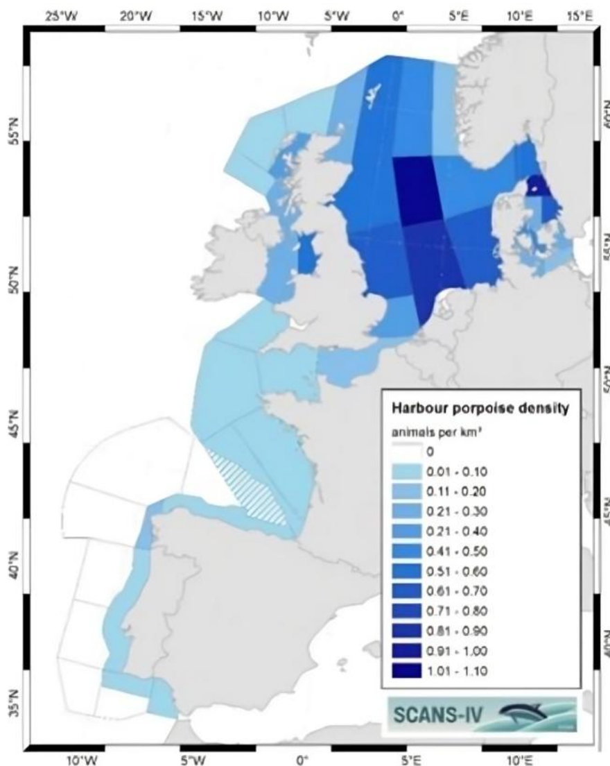
Figure 3-1: Predicted density surface for harbour porpoise in 2022 using SCANS IV survey data.
