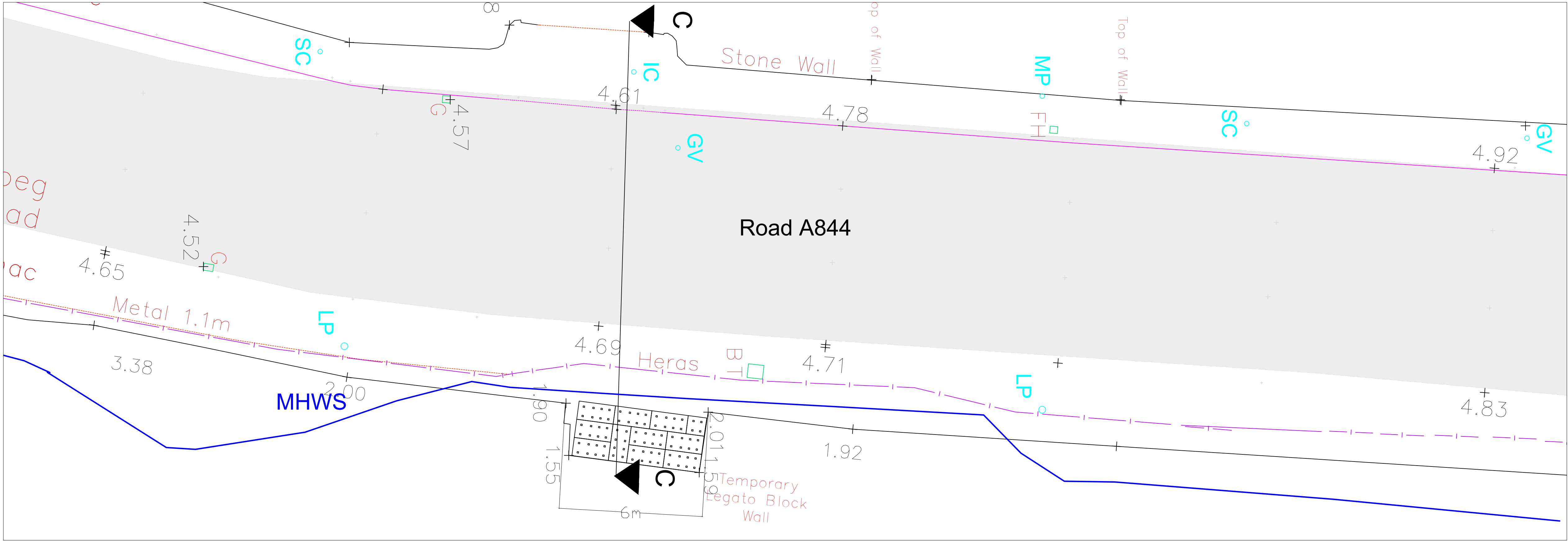
Existing Plan Seawall 1 Scale 1:100
