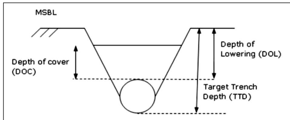
Figure 5.18 – Key as-trenched measured parameters
