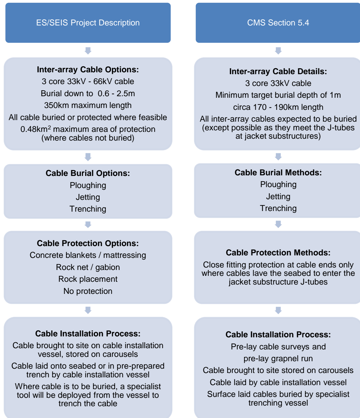
Figure 7.3 – Comparison of inter-array cable installation methods described in the ES/SEIS and CMS
