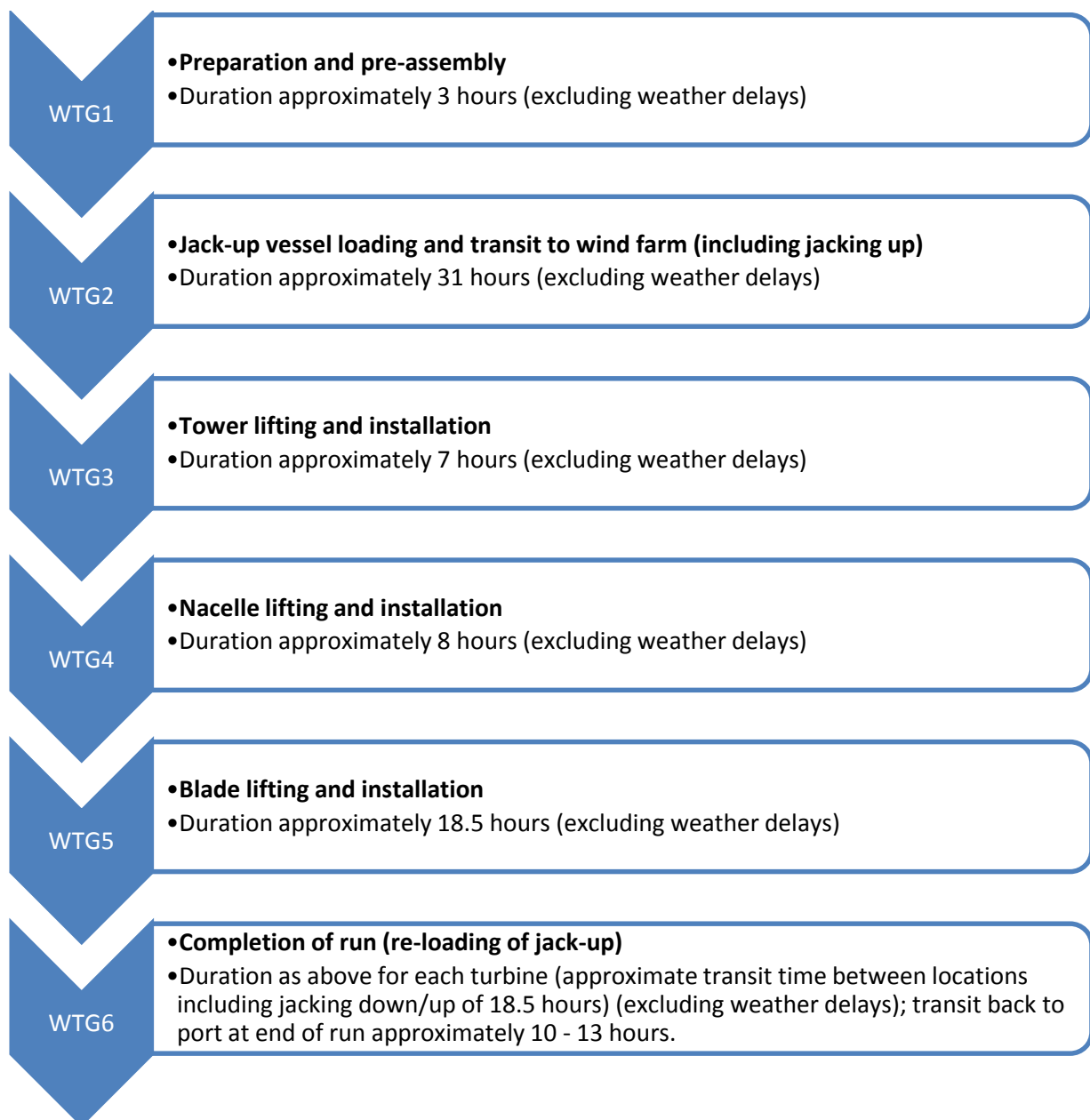
Figure 5.19 Wind Turbine Installation Sequence
