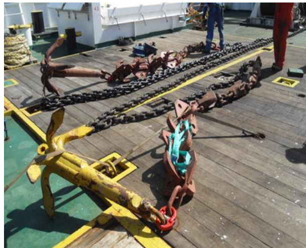
Figure 5.14 - Example of a grapnel that may be used for the PLGR
