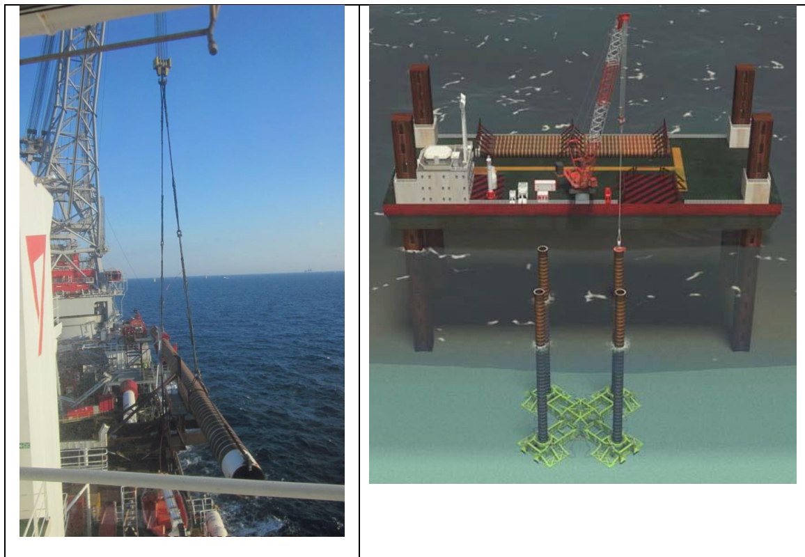
Figure 5.6 – Pile being up-ended ready for deployment and being deployed into the PIF
