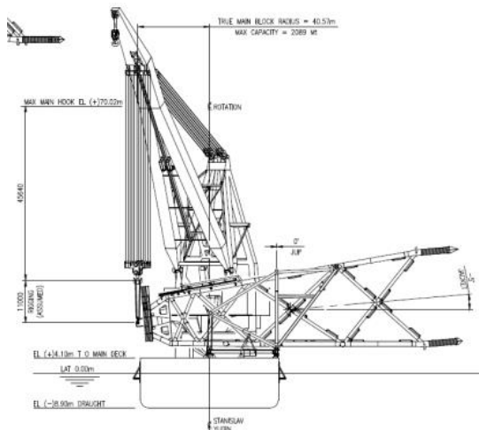
Figure 5.10 – Lifting of a horizontally mounted jacket substructure
