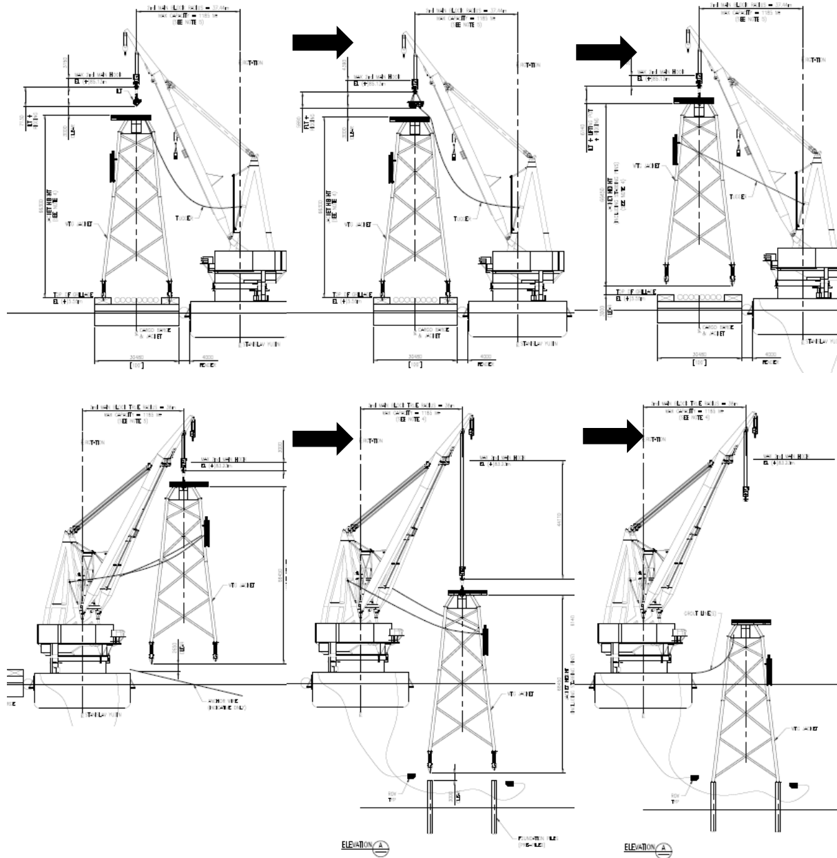
Figure 5.11 - Example of sequential jacket installation procedure for a vertically mounted jacket substructure
