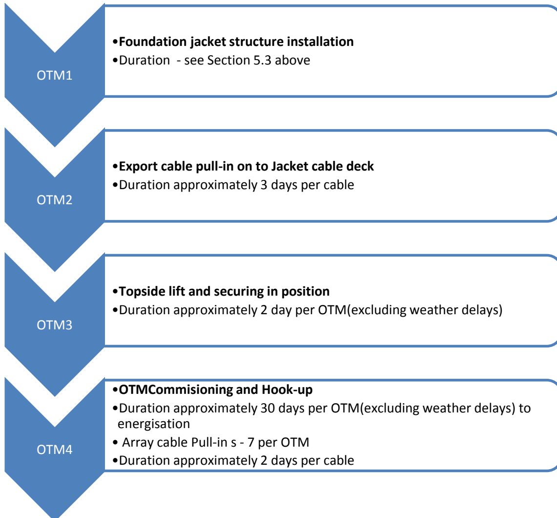
Figure 5.24 OTM Installation Sequence
