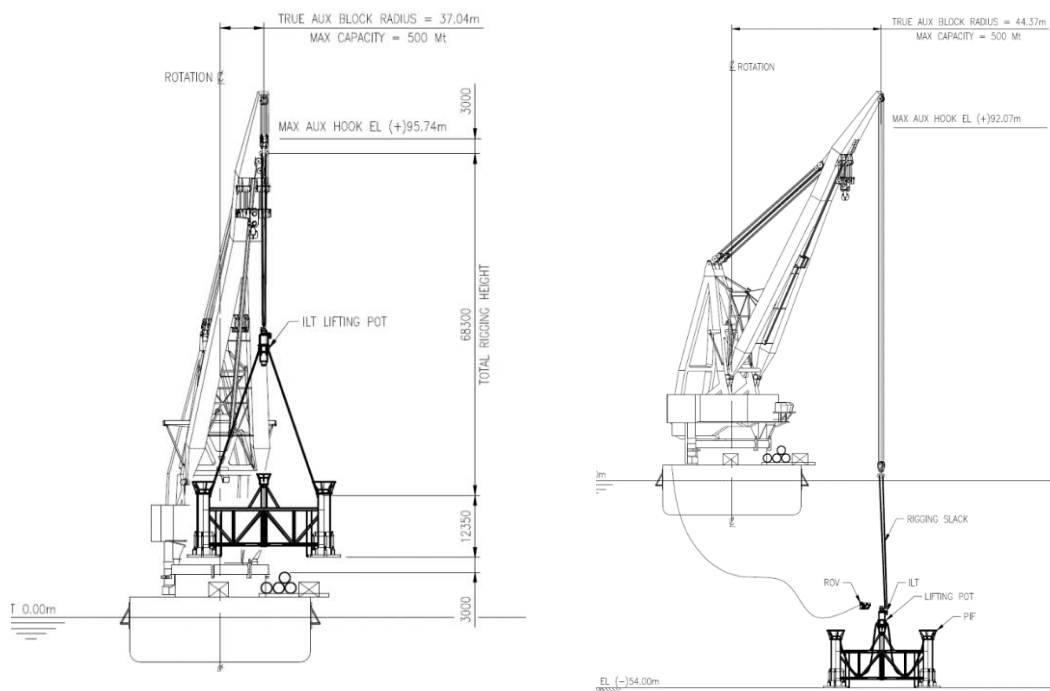
Figure 5.5 – PIF being lifted from the deck of the HLV for lowering to the seabed
