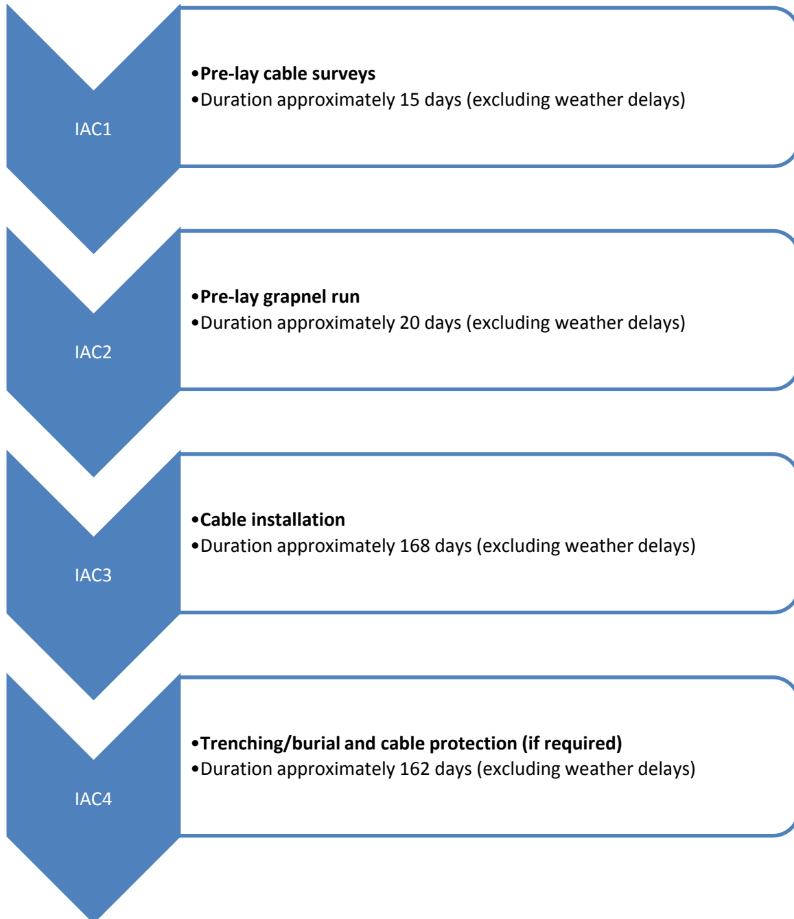
Figure 5.13 Inter-array Cable Installation Sequence
