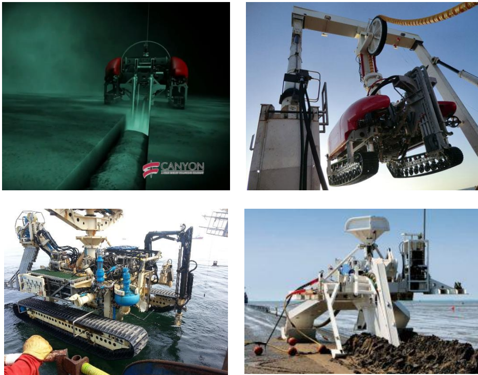
Figure 5.16 – Examples of seabed water jetting cable trenching tools and cable plough that may be used for inter-array cable installation
