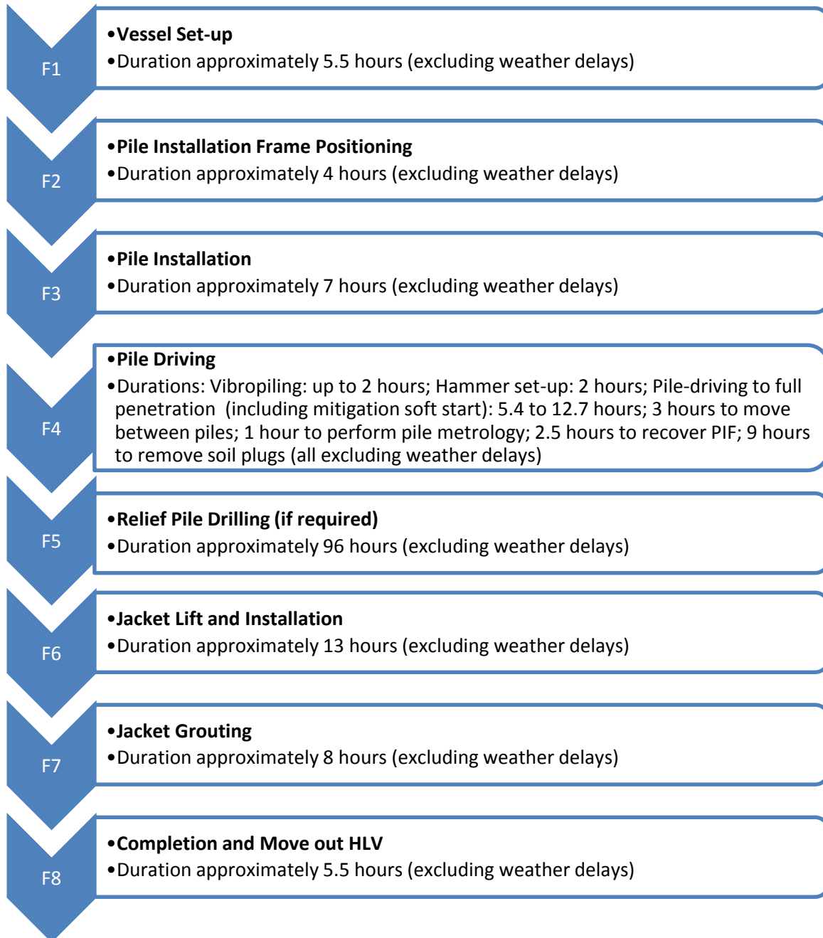
Figure 5.3 Jacket Foundation and Substructure Installation Sequence
