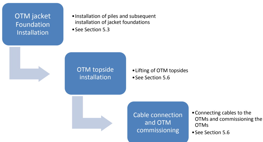
Figure 5.2 – Overview of OTM installation process
