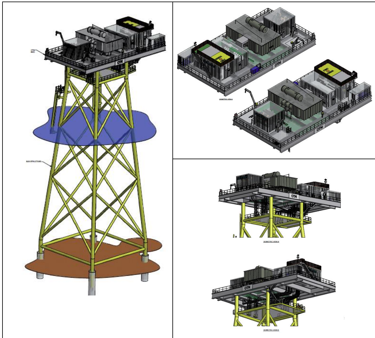
Figure 5.25 - Example of an OTM top-side layout installed on a jacket structure and arrangements of topsides and cable deck
