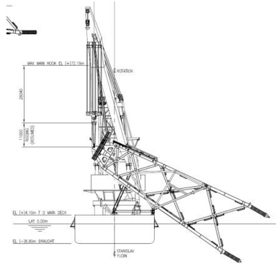
Figure 5.10 – Lifting of a horizontally mounted jacket substructure
