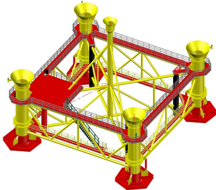
Figure 5.4 – Example of a Hydraulically Operated PIF
