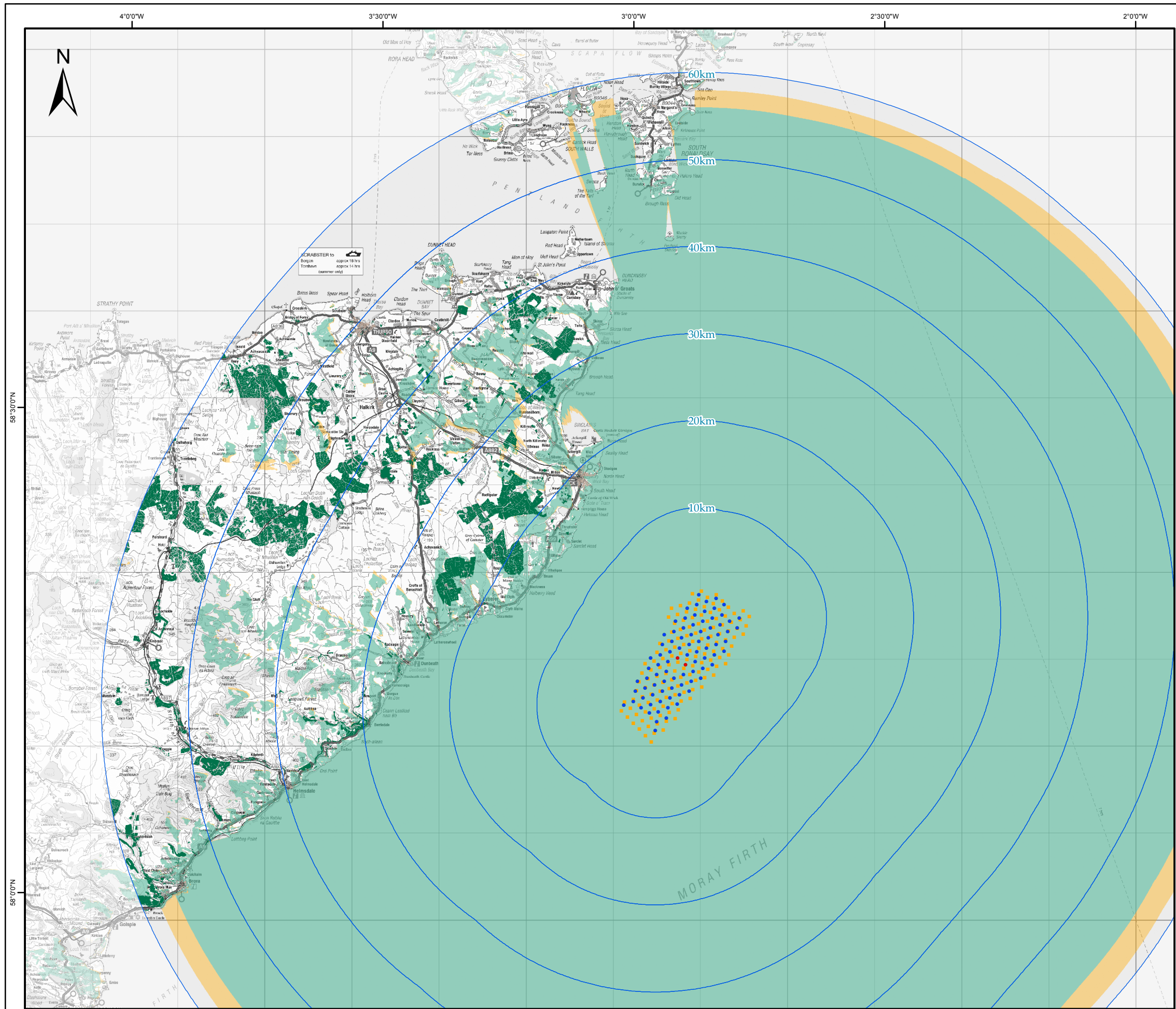
UK Offshore Development Figure 03 Zone of Theoretical Visibility Final and Consented Layouts - with Screening
