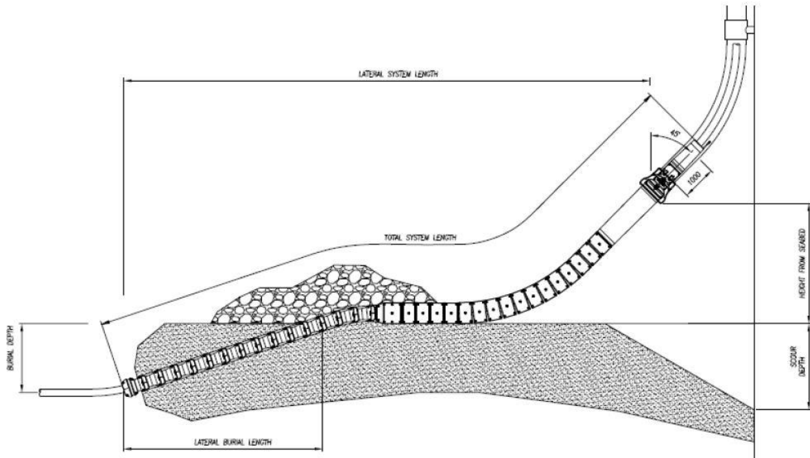
Figure 16 Example of a CPS at a J-tube
