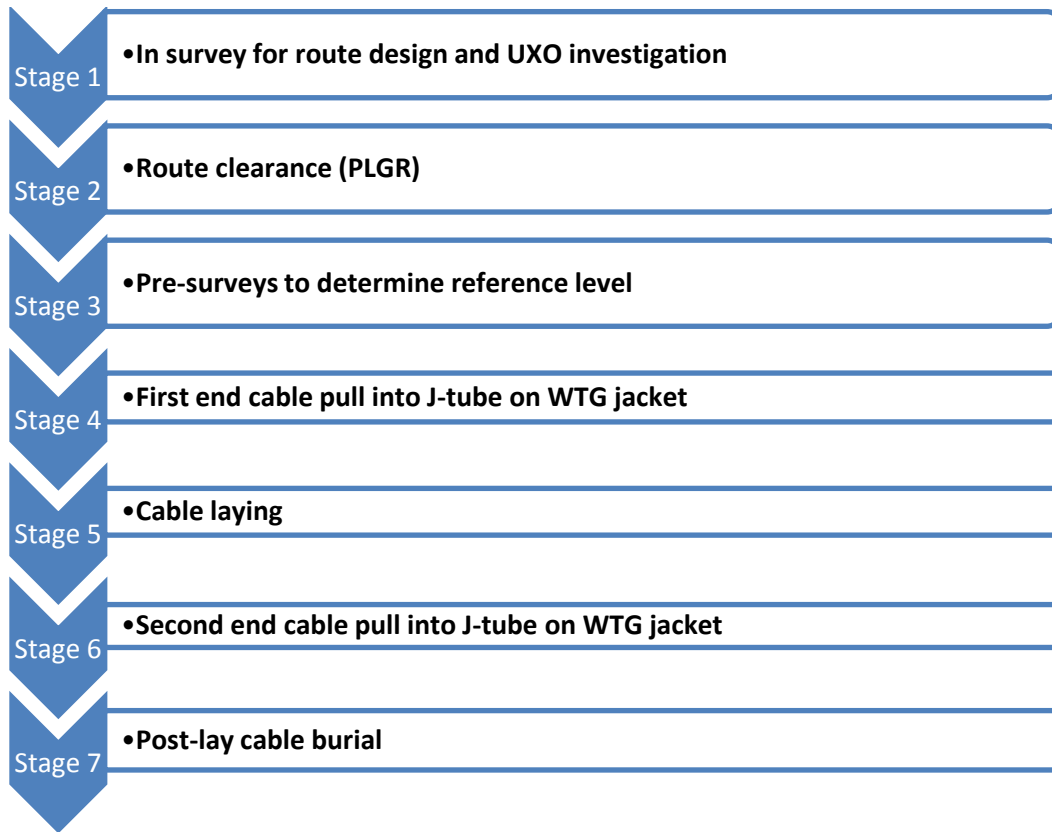
Figure 20 Inter-array Cable Installation Sequence
