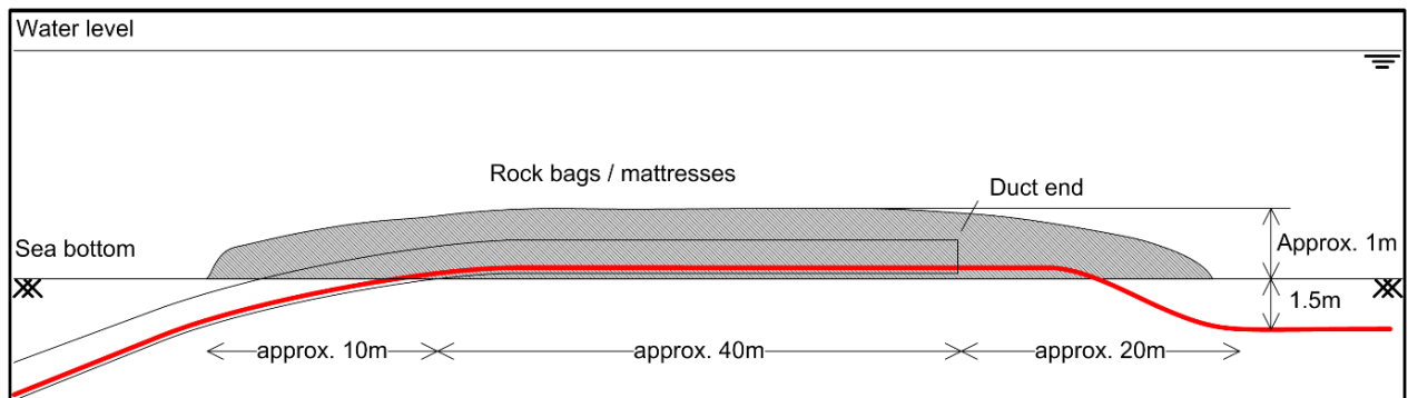
Figure 17 Indicative duct and cable protection
