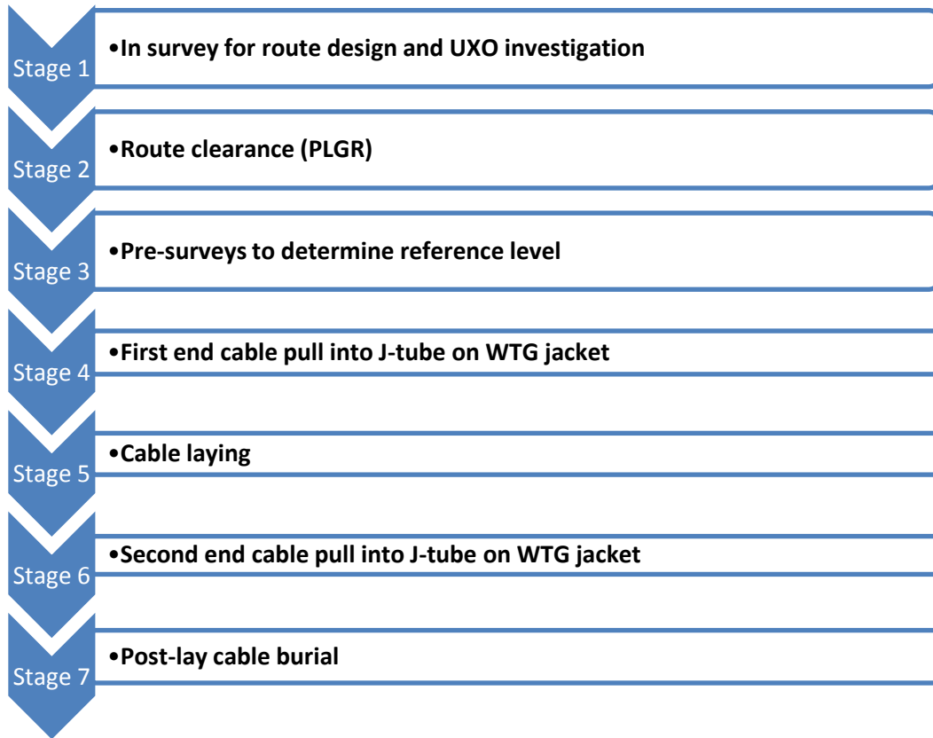
Figure 16 Inter-array Cable Installation Sequence
