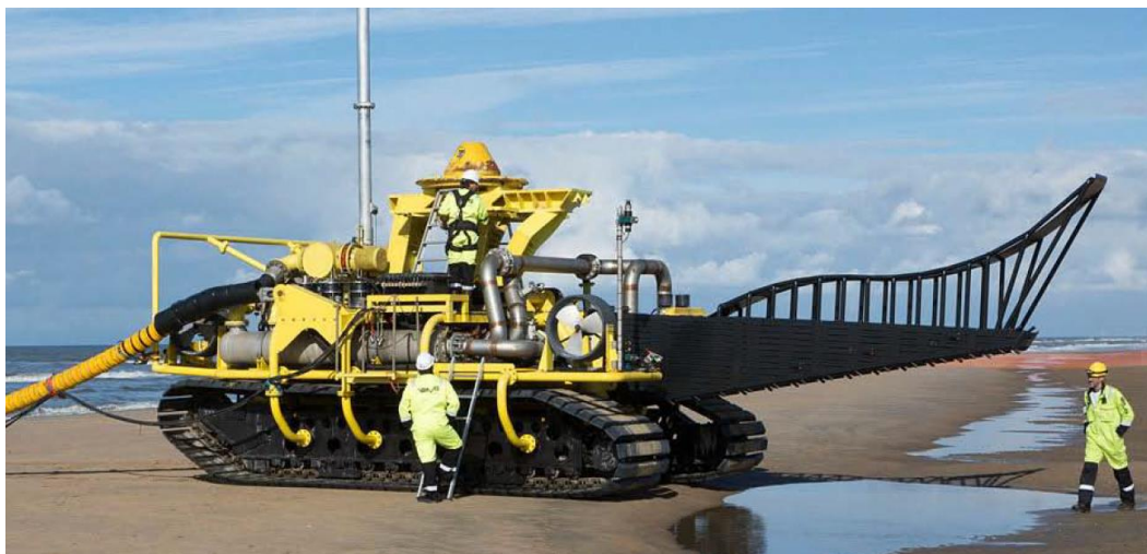
Figure 12 Examples of seabed cable trenching tools (cutting and jetting)
