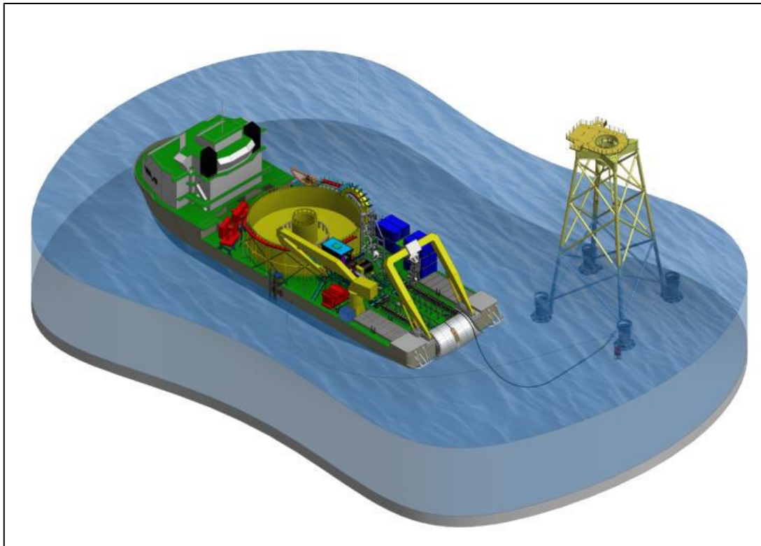
Figure 17 First end cable pull in
