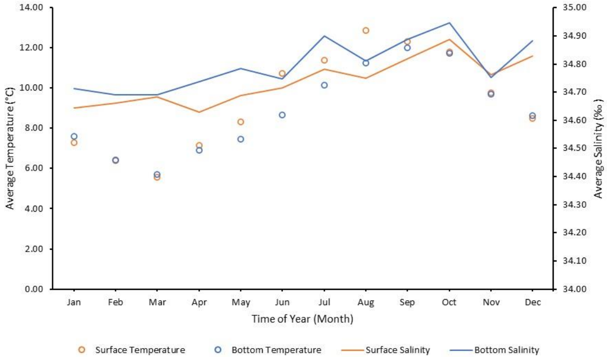
Figure 2-2: Monthly mean sea surface and bottom temperature and salinity across the Caledonia North OECC based on climatology data between 1971 and 2000. Source: Marine Directorate (2024 1 ).
