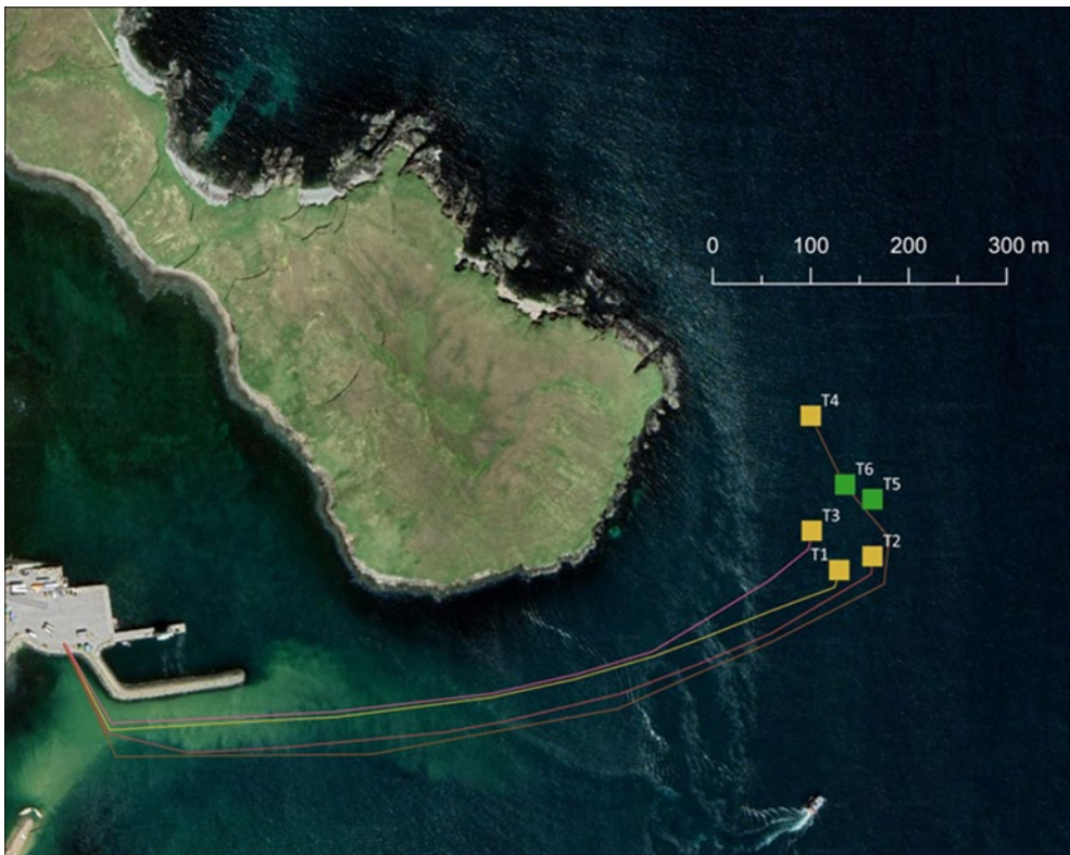
Figure 2-2: Shetland Tidal Array installed layout, including six turbines and five export cables.
