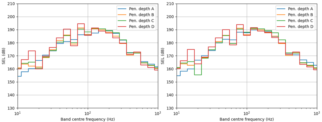
Figure 6.4: Morven South: Maximum-over-depth per-pulse Sound Exposure Level in decidecade bands, 10m from the pile centre for the 3.7m pin pile in median reflectivity environment (left) and maximum reflectivity environment (right)
