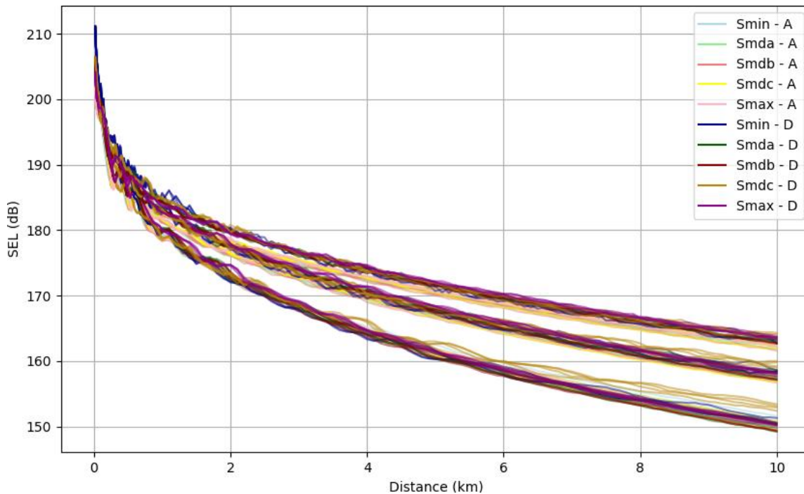
Figure A.5: Per-pulse Sound Exposure Level as a function of distance of the 16.0m monopile split by location and analysis depth for Morven North (top) and Morven South (bottom). Colours distinguish the different source locations and the analysed penetration depth (A: shallowest; D: deepest)
