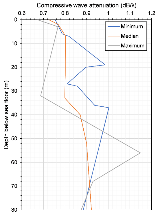
Figure A.4: Compressive wave attenuation associated with each of the minimum, median, and maximum profiles for sensitivity studies
