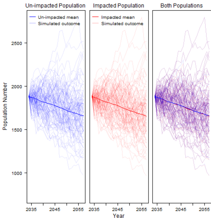
Figure 3.5: Simulated population trajectories in an unimpacted versus impacted population for the maximum temporal scenario for the Greater North Sea MU bottlenose dolphin population
