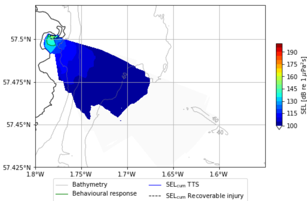
Figure 4.14 SEL levels and impact ranges predicted for fish with a swim bladder during rock breaking at the Peterhead harbour
