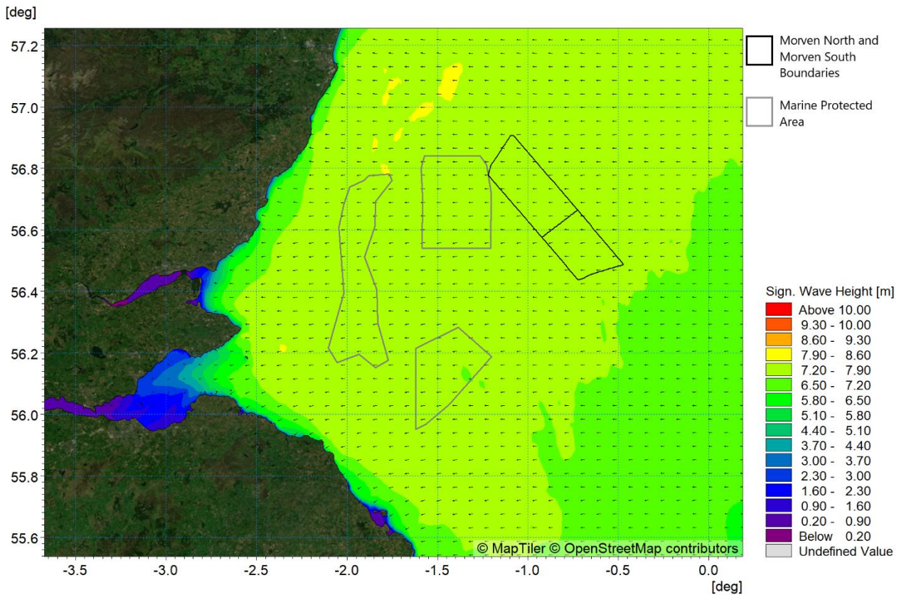
Figure 4.48: Wave climate 1:1 year storm from 090° at mid-tide
