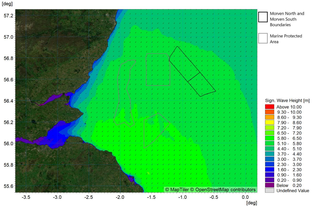
Figure 4.47: Wave climate 1:1 year storm from 045° at mid-tide
