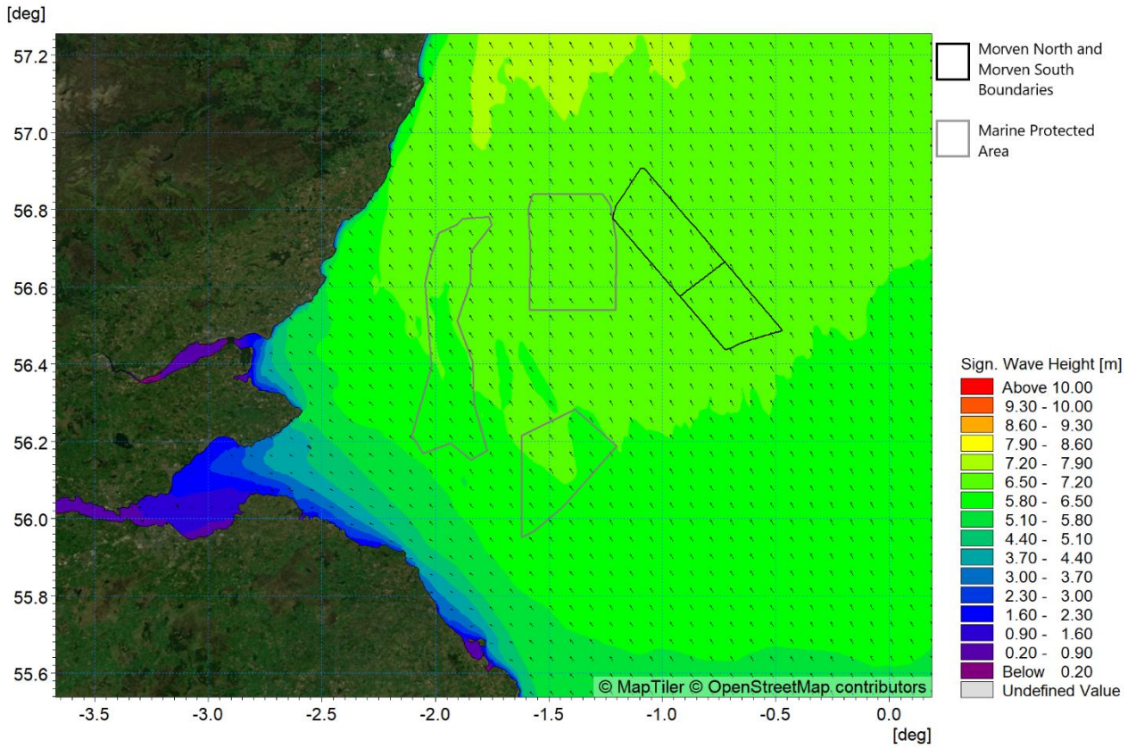
Figure 4.49: Wave climate 1:1 year storm from 135° at mid-tide
