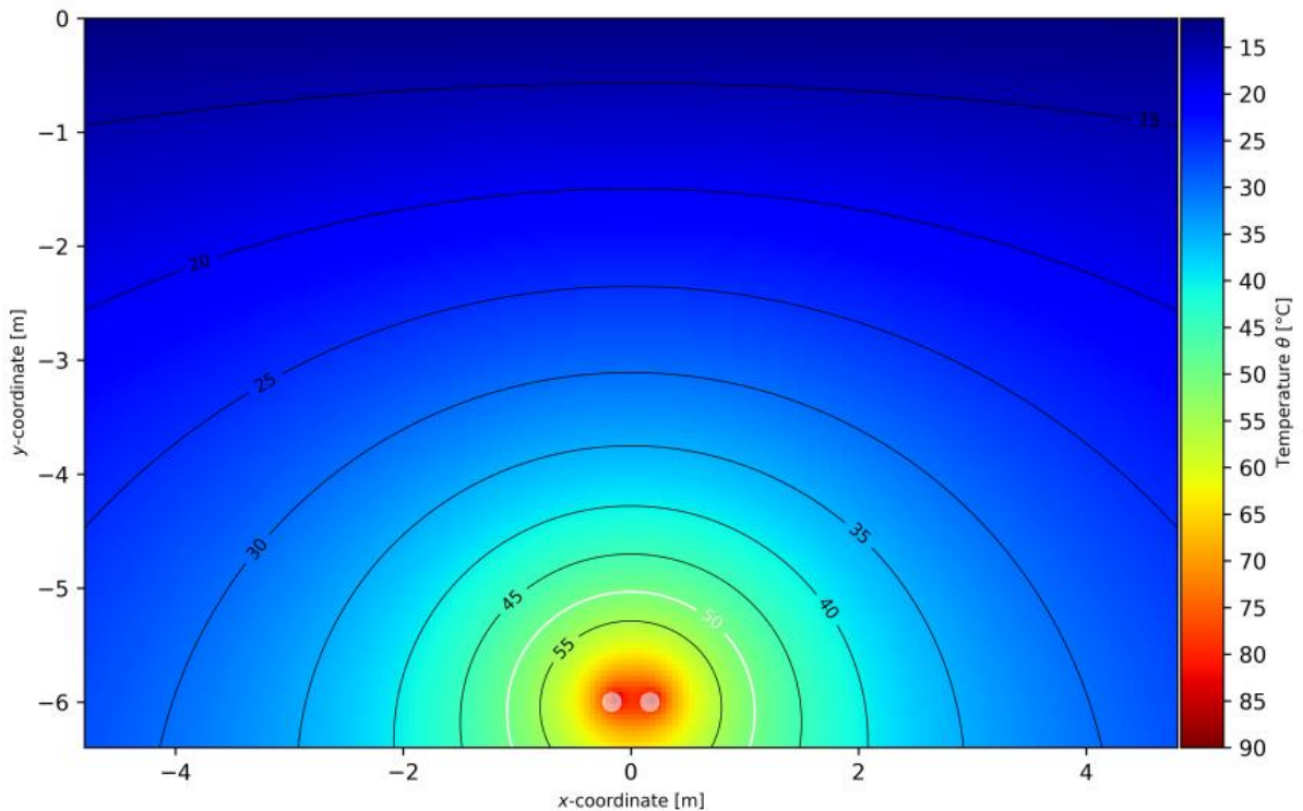
Figure 7: Heat Plot for Case 7 – Cables in Seabed Below Sandwave – Temperature Constrained
