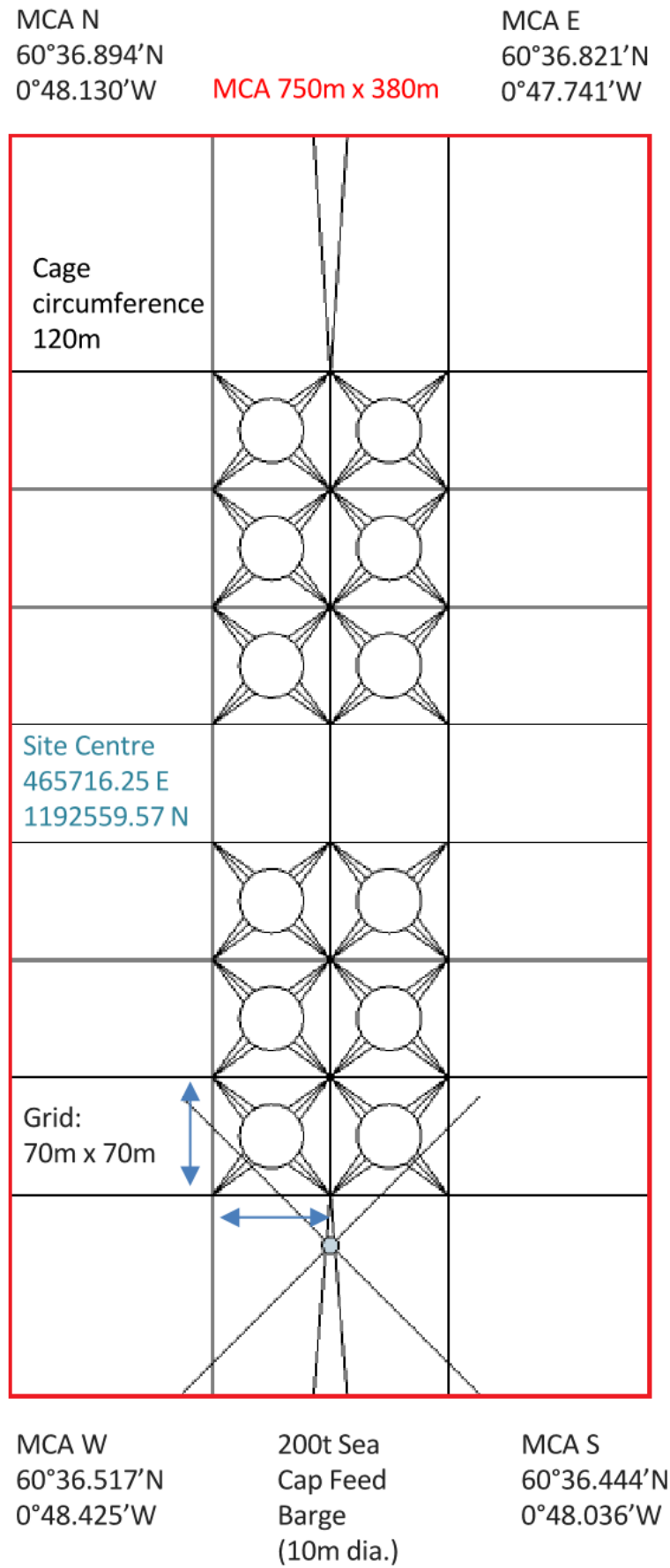
Wick of Gruting Site Plan
